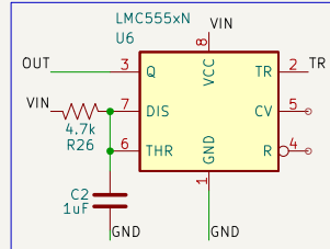
Monotable 555 Timer
