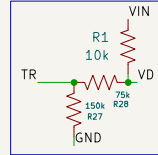
Voltage Divider
