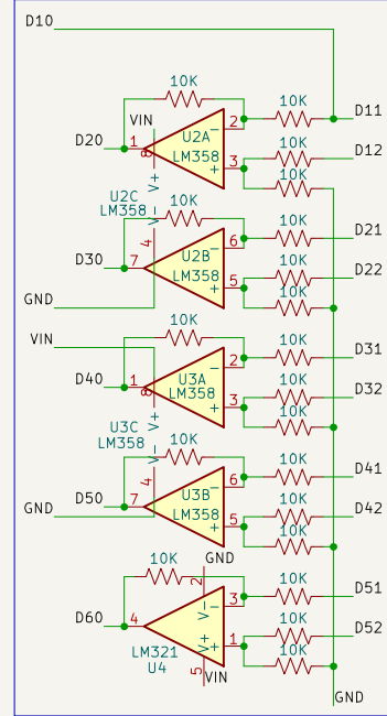
Differential Op-Amp Array
