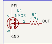
Mosfet Driver (for relay)
