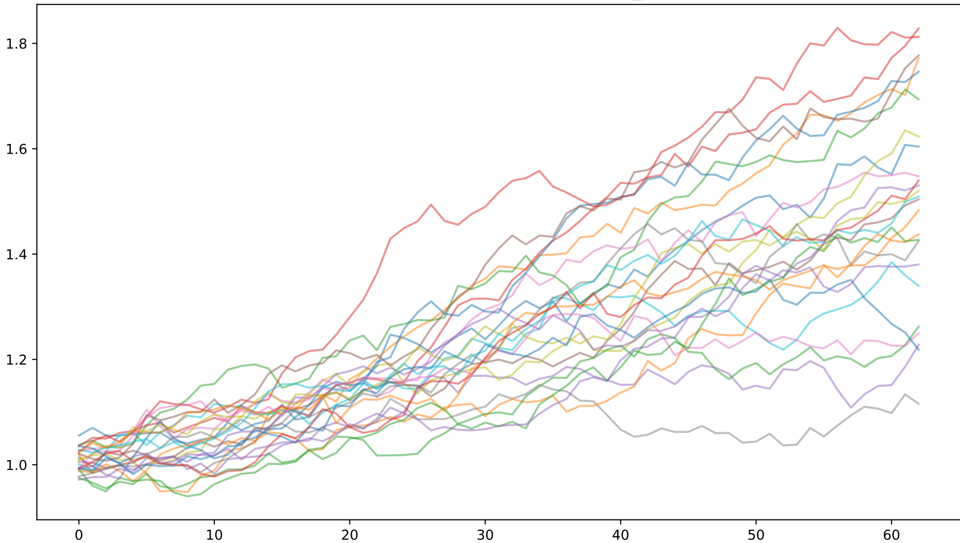
Monte Carlo Price Paths (Sample, mv_ml)
