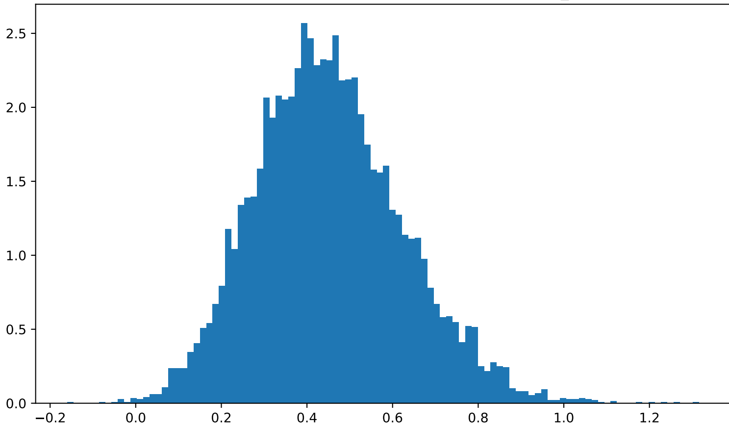
Sample Monte Carlo Final Return Distribution (mv_ml)
