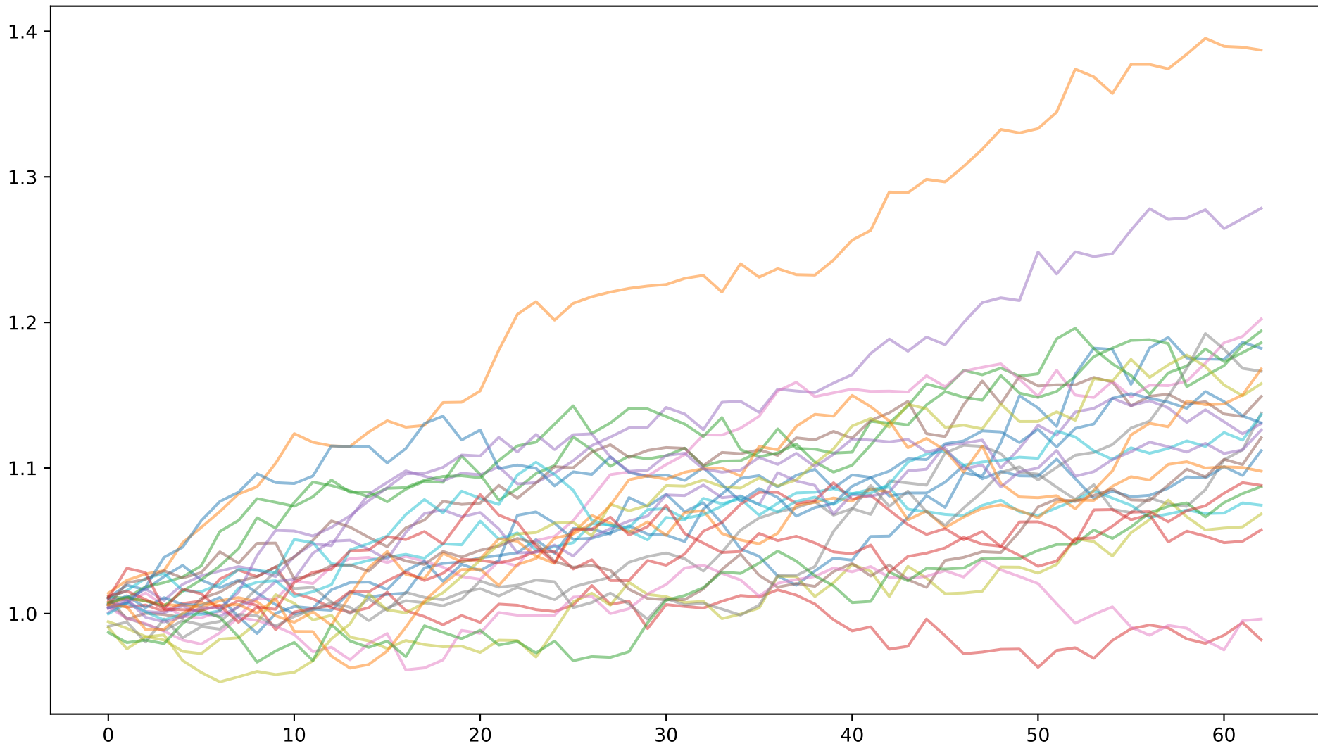
Monte Carlo Price Paths (Sample, eq)
