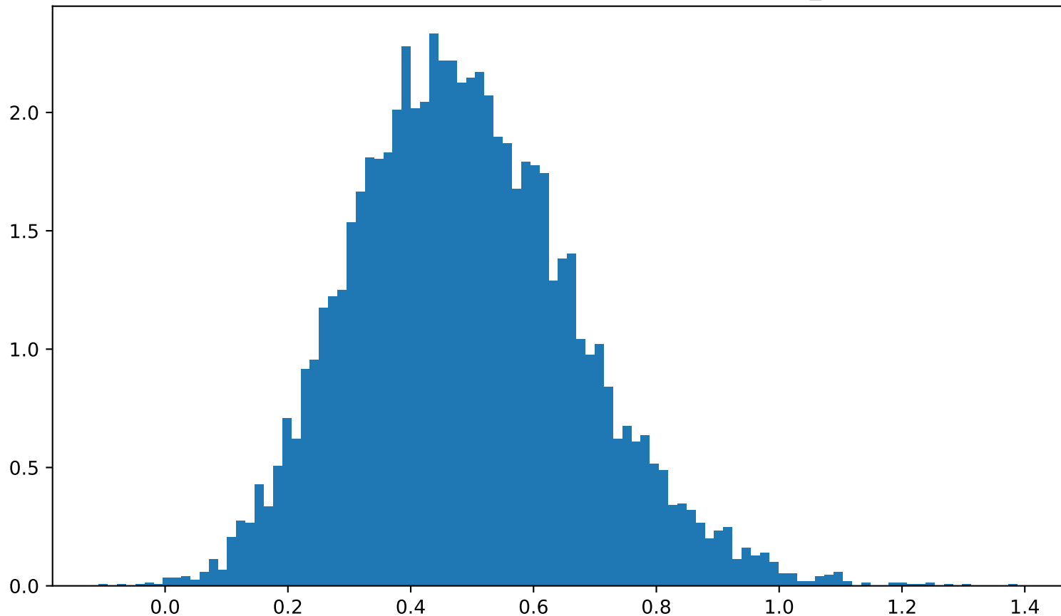
Sample Monte Carlo Final Return Distribution (mv_hist)
