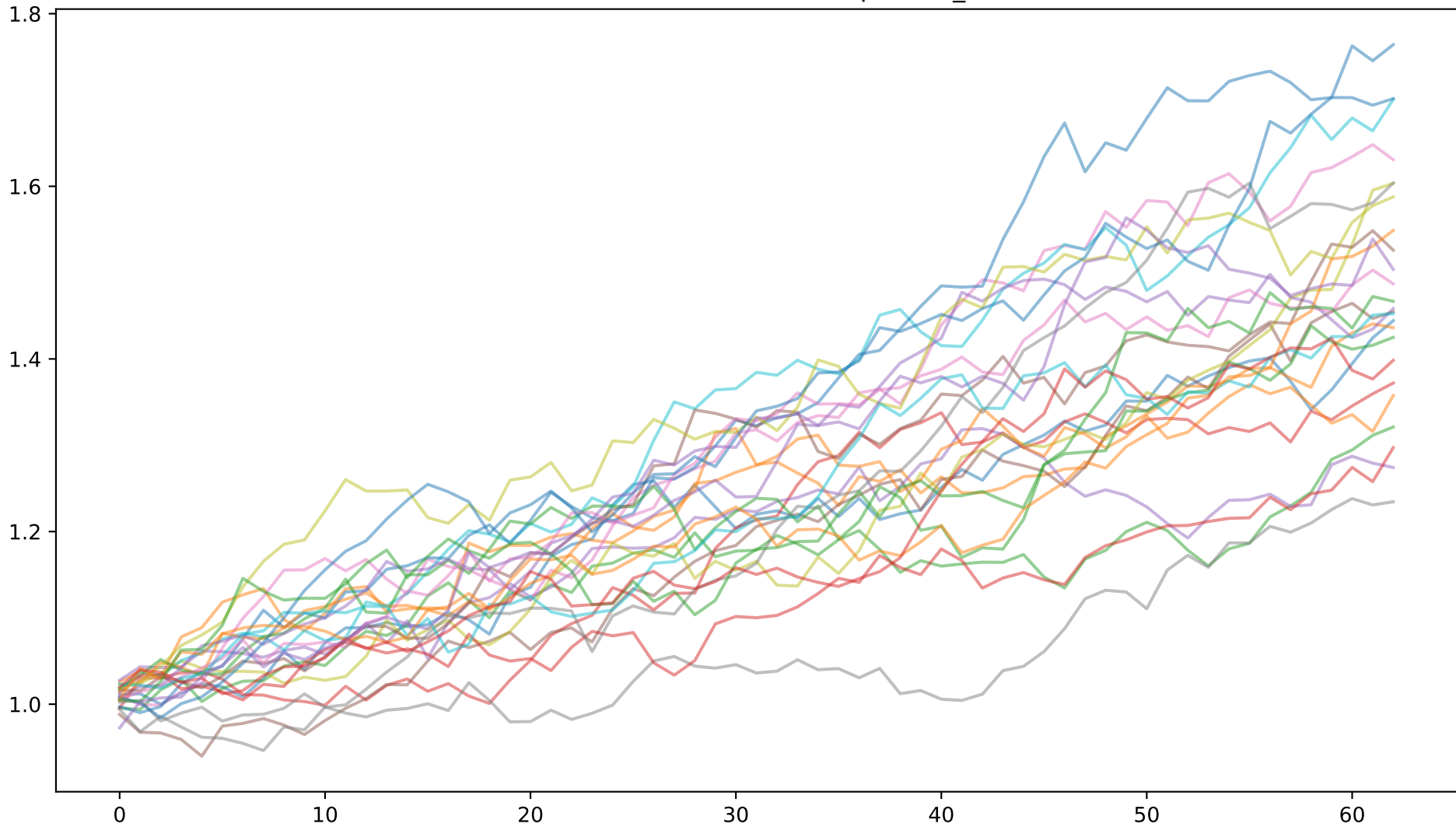
Monte Carlo Price Paths (Sample, mv_hist)
