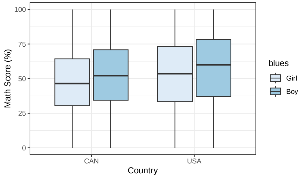
Math Scores by Country and Sex
