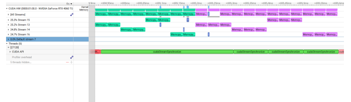
Fig. 7. Detailed Nsight Systems view of stream usage in a non-filtering stage.
