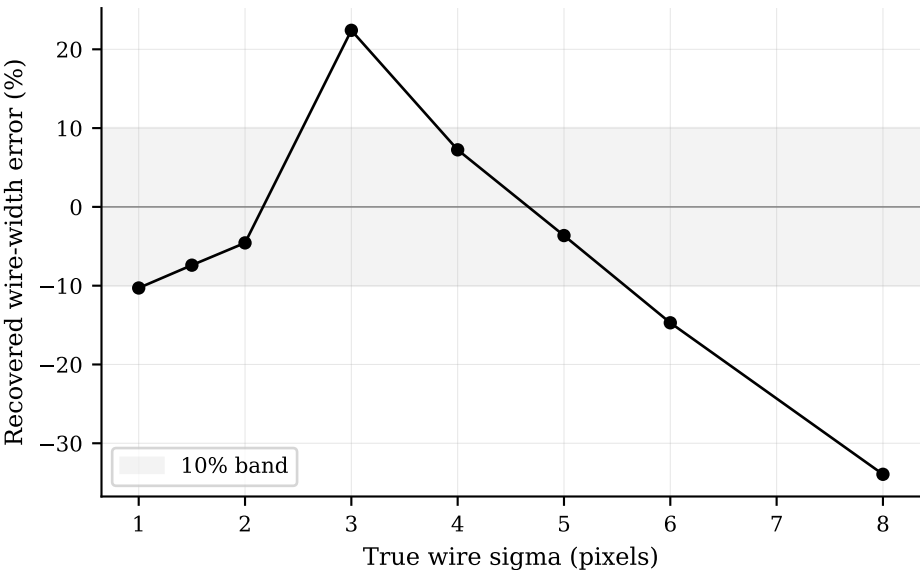
Wire-width sweep on synthetic phantom
