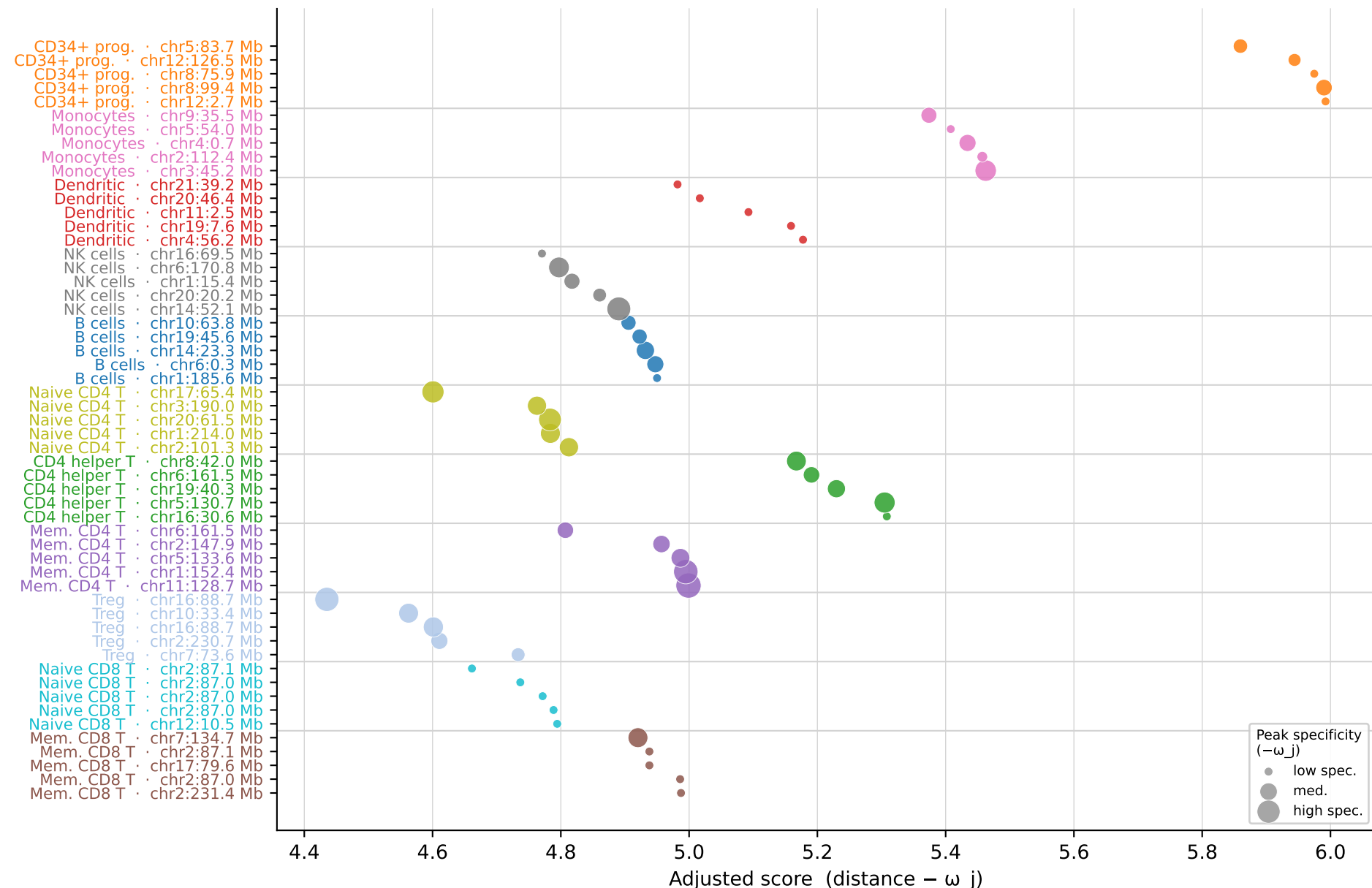
Top 5 marker peaks per cell type ranked by adjusted centroid distance Dot size = peak specificity ( -\omega_j ); smaller score = stronger marker
