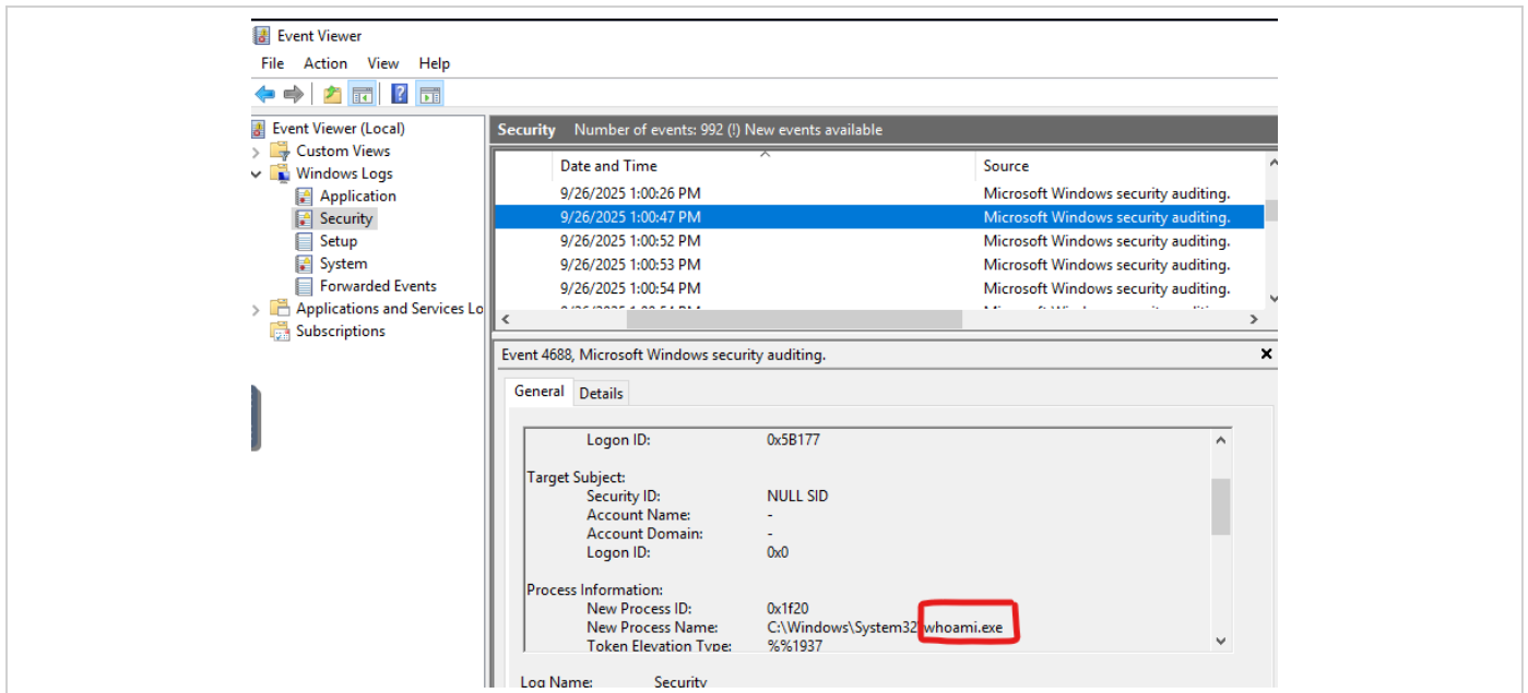
Event Viewer — Event ID 4688 showing execution of whoami.exe
