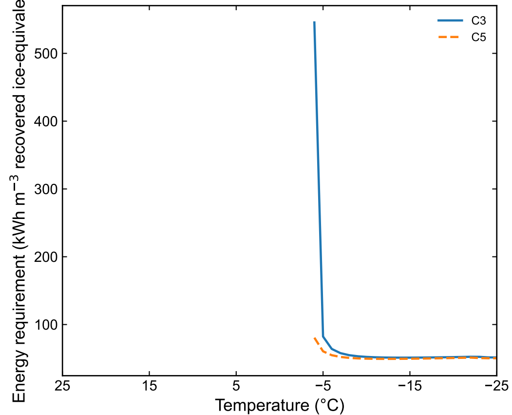
(a) Refrigeration energy vs temperature
