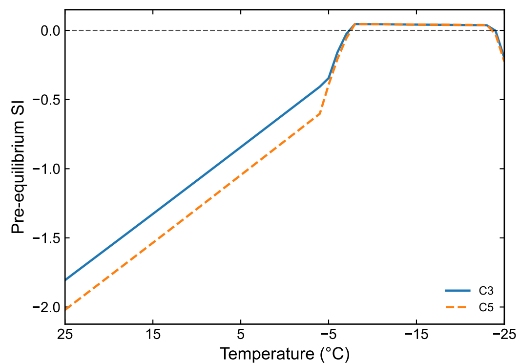
(b) Mirabilite saturation
