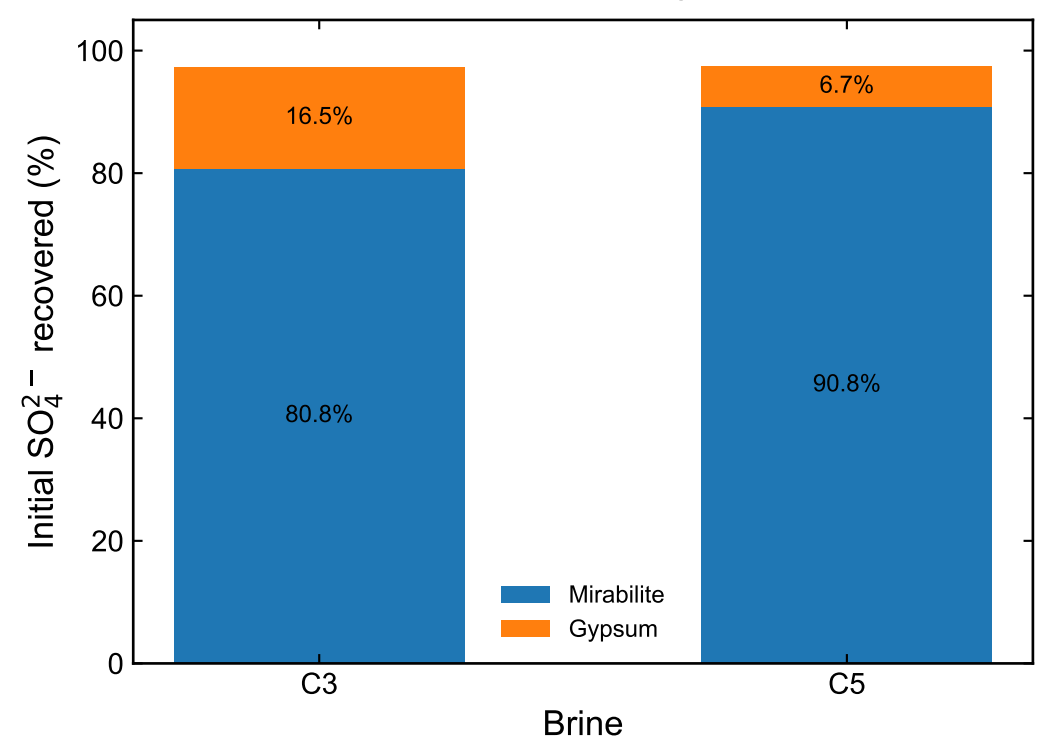
(f) Sulphate partitioning at -25 °C
