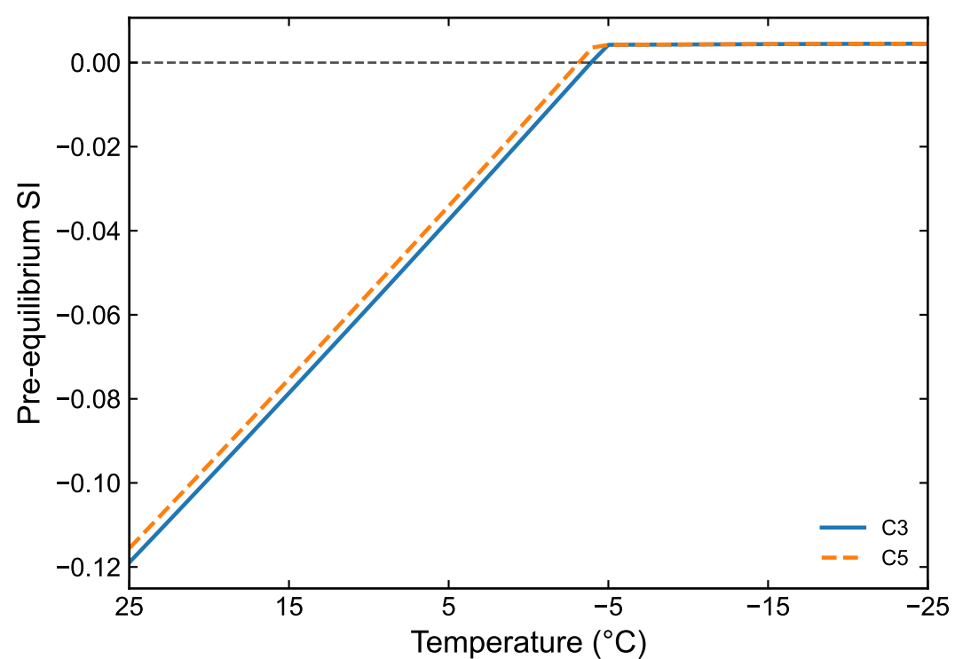
(a) Ice saturation
