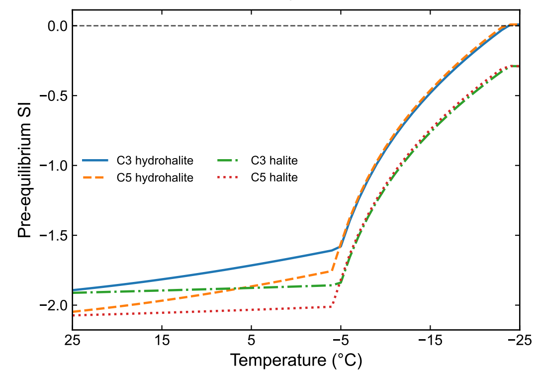
(c) NaCl-bearing phase saturation
