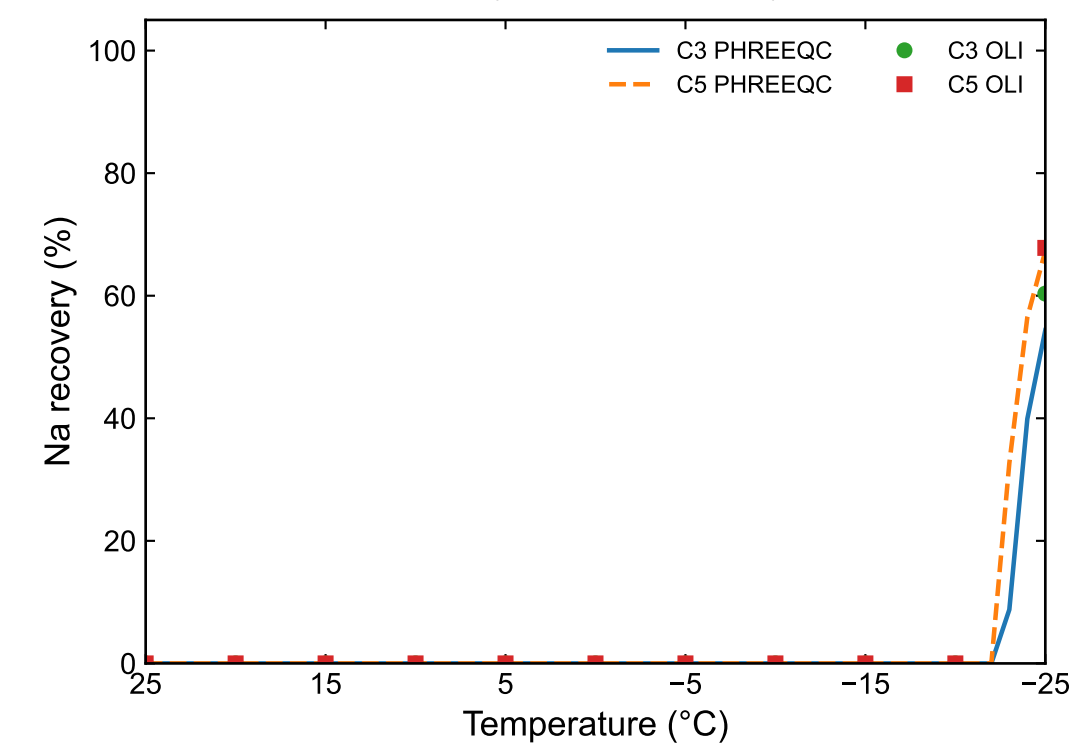
(e) Hydrohalite recovery
