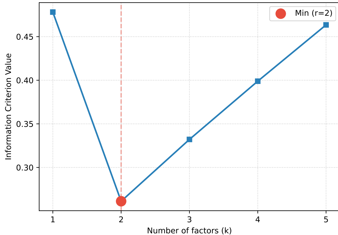
ICp2 Criterion (Bai & Ng)
