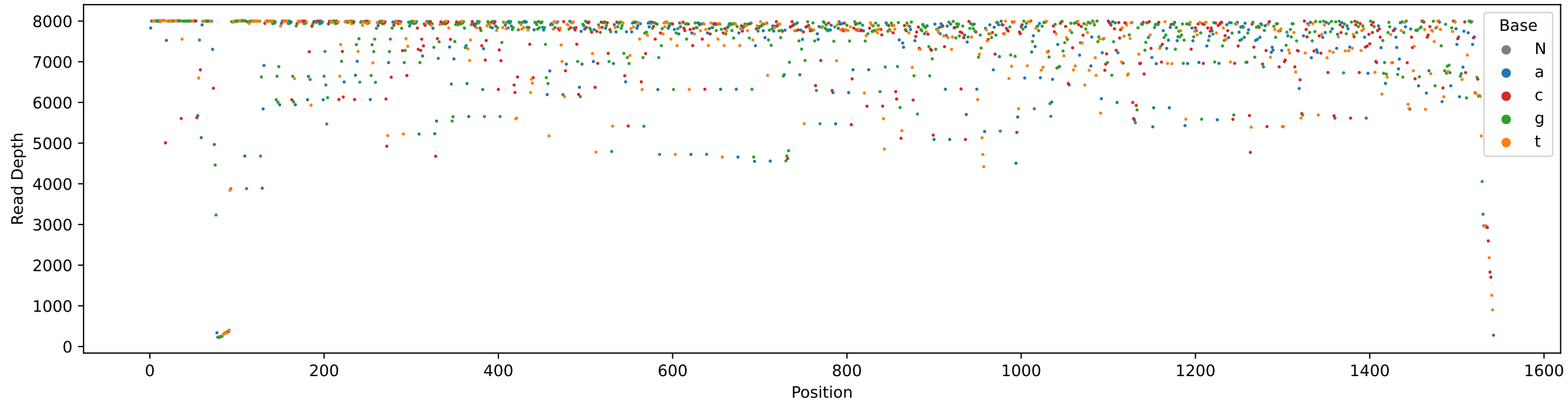
SRR10533475.sorted_depth - 16S_consensus Coverage
