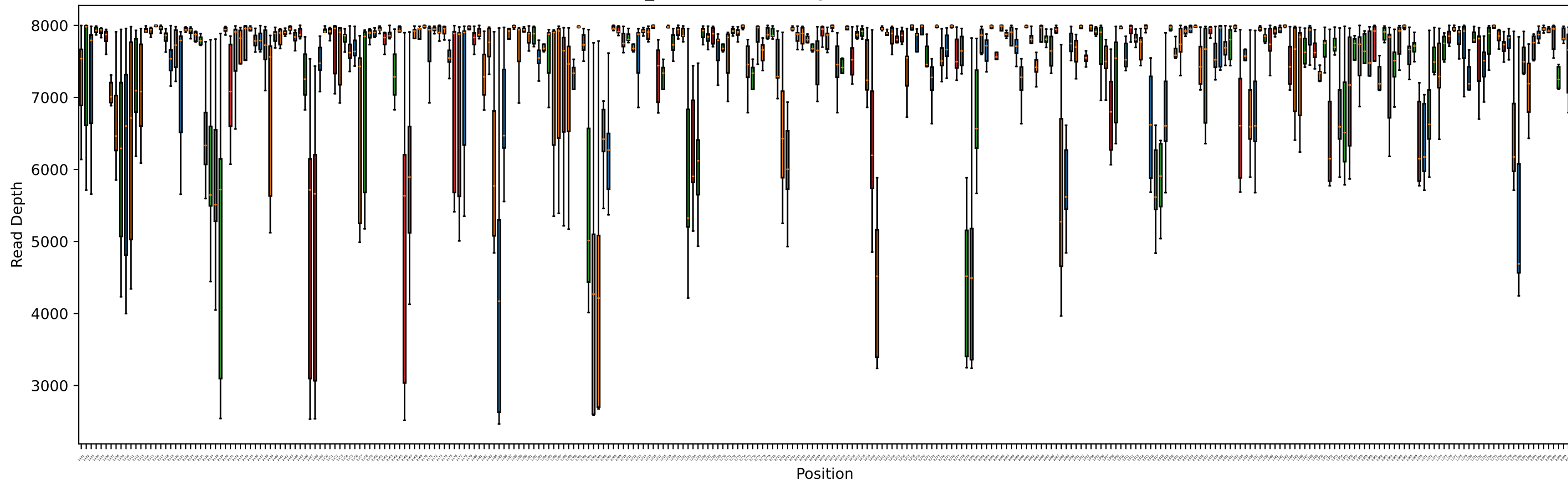
23S_consensus Coverage - Positions 2101-2400
