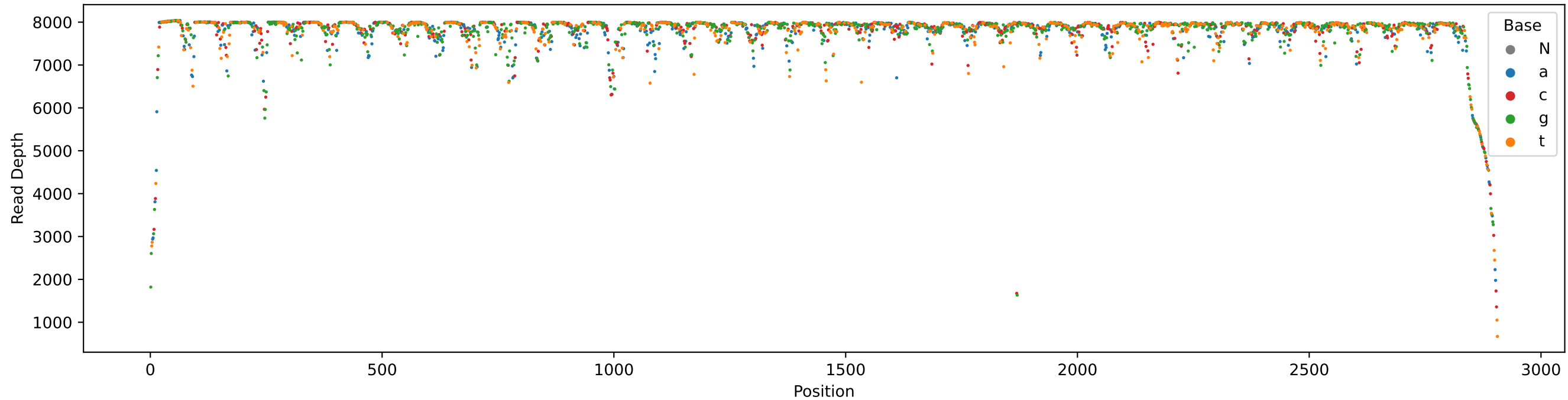
SRR11584025.sorted_depth - 23S_consensus Coverage
