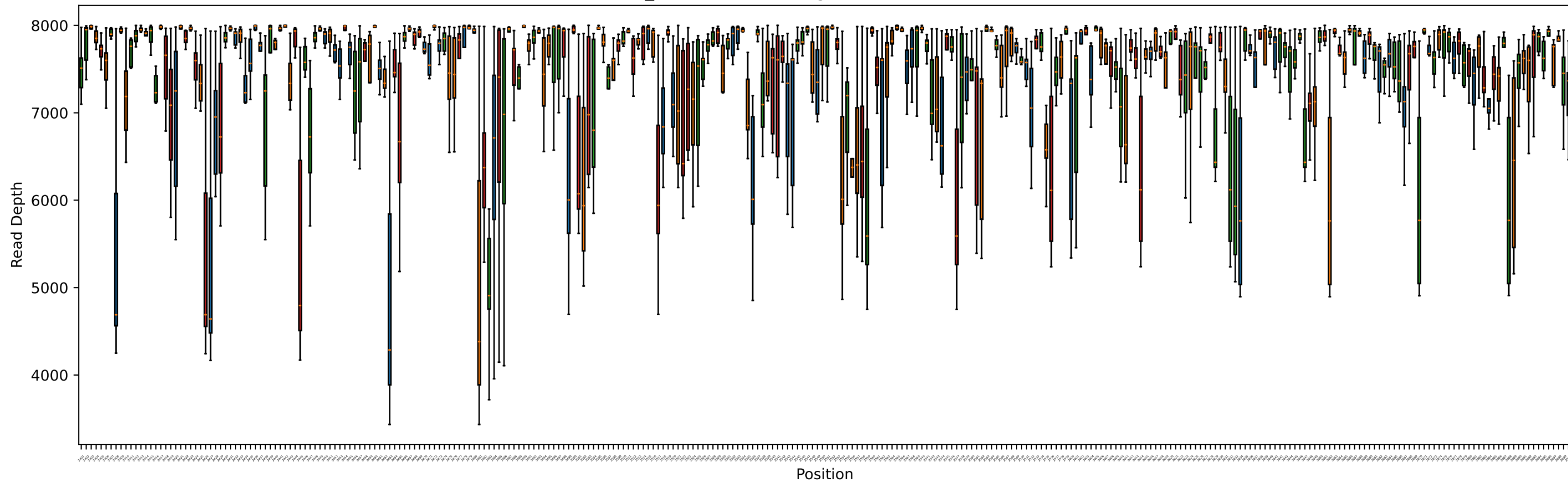
23S_consensus Coverage - Positions 2401-2700
