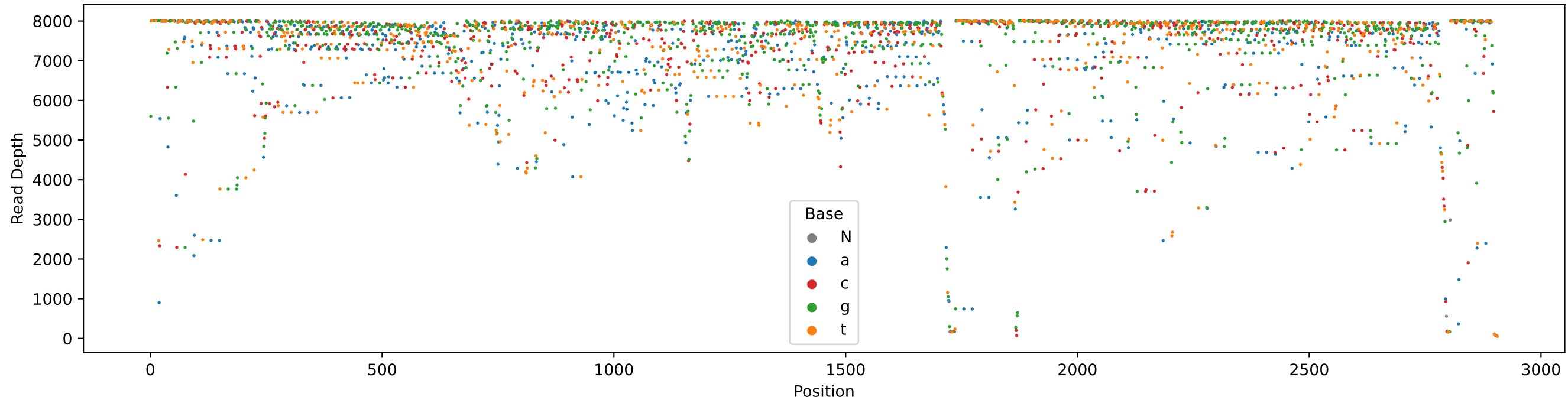
SRR11584024.sorted_depth - 23S_consensus Coverage
