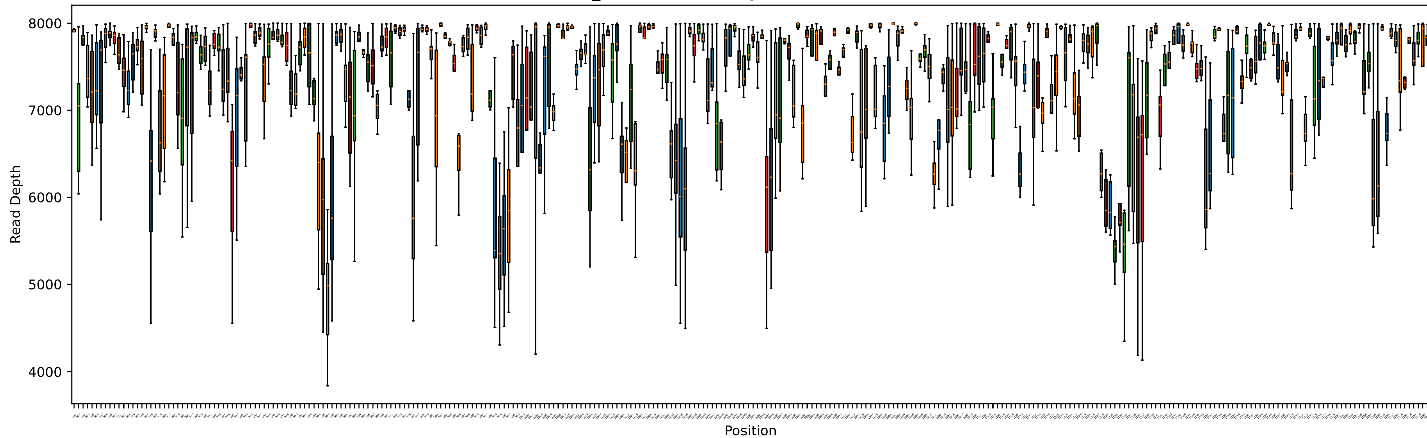
16S_consensus Coverage - Positions 901-1200
