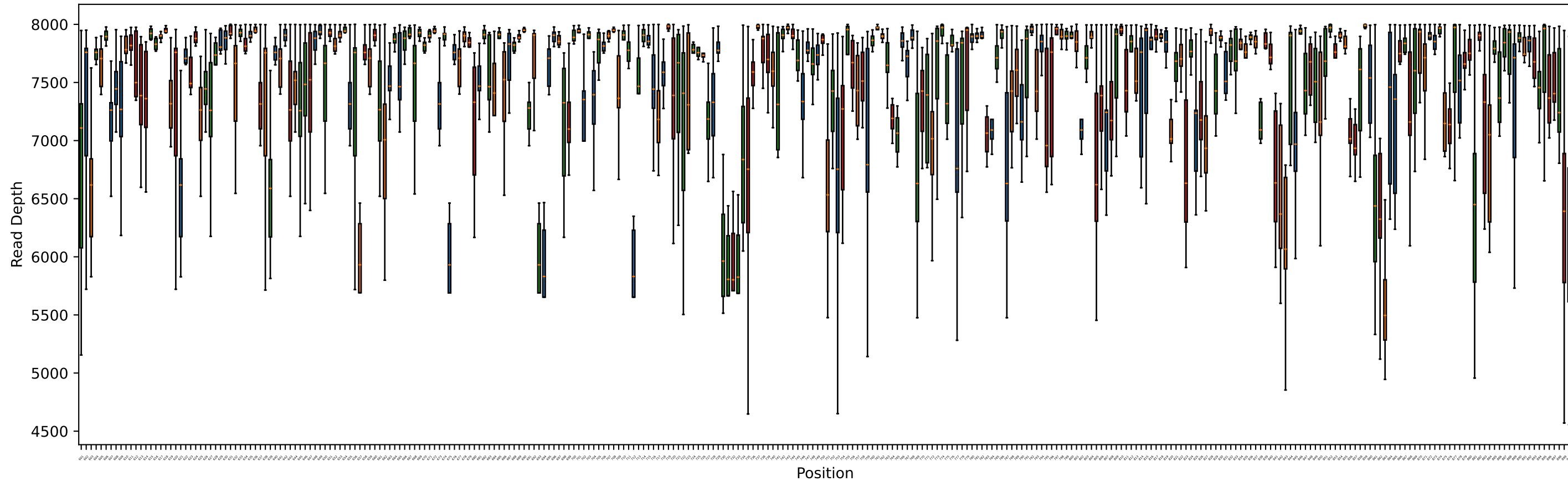
16S_consensus Coverage - Positions 601-900
