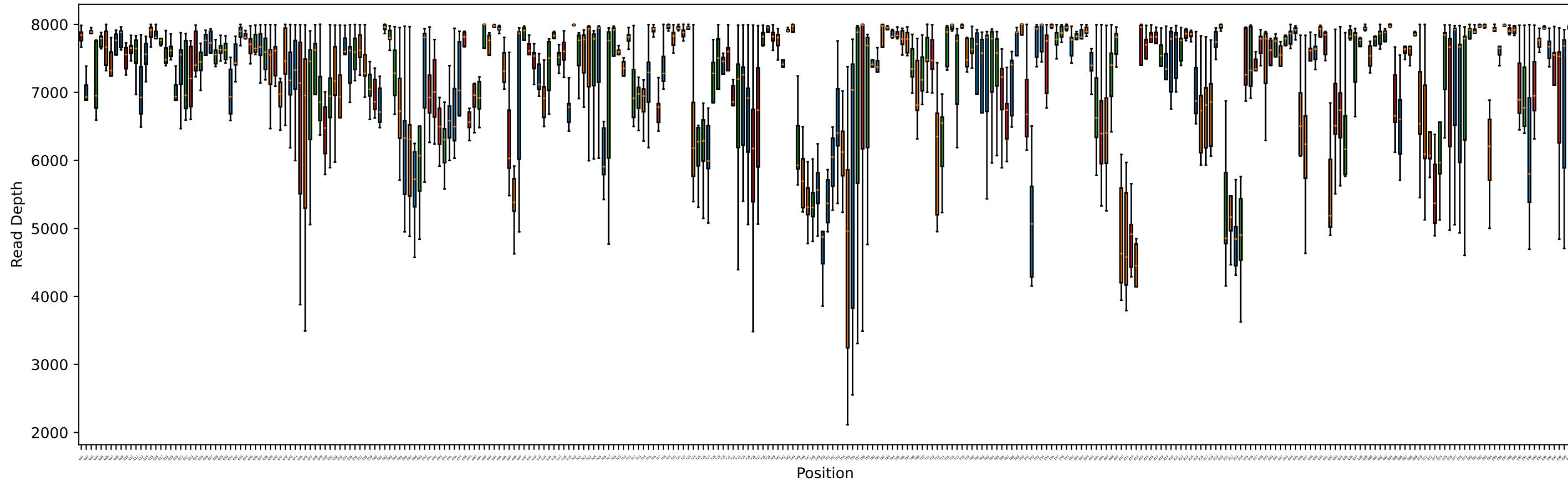
23S_consensus Coverage - Positions 601-900
