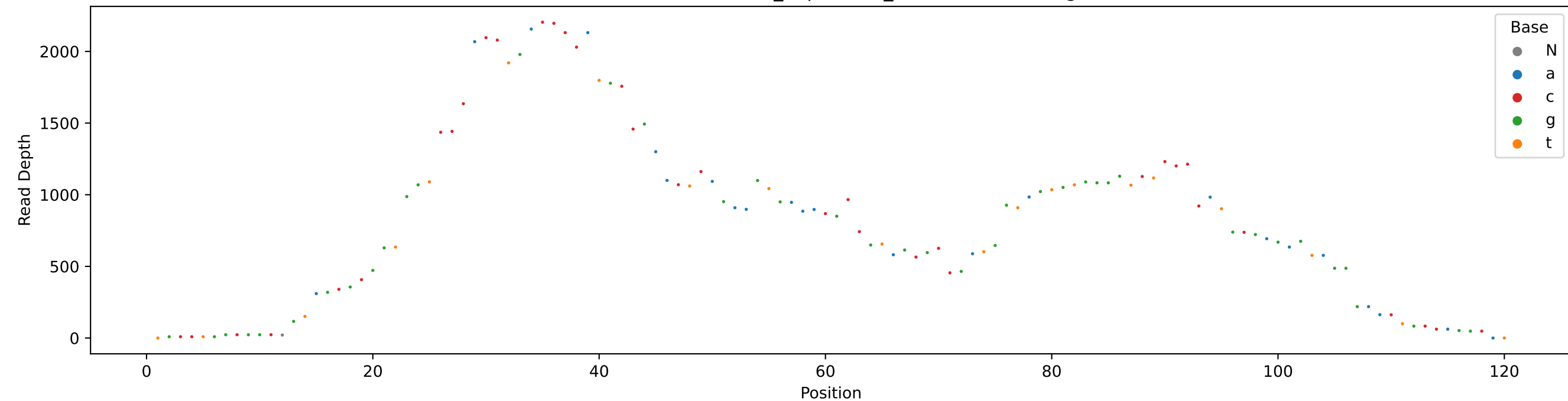
SRR11584028.sorted_depth - 5S_consensus Coverage
