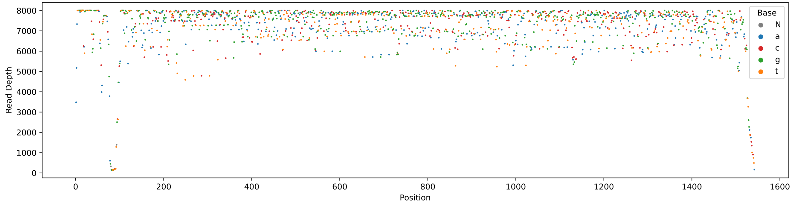
SRR10533474.sorted_depth - 16S_consensus Coverage
