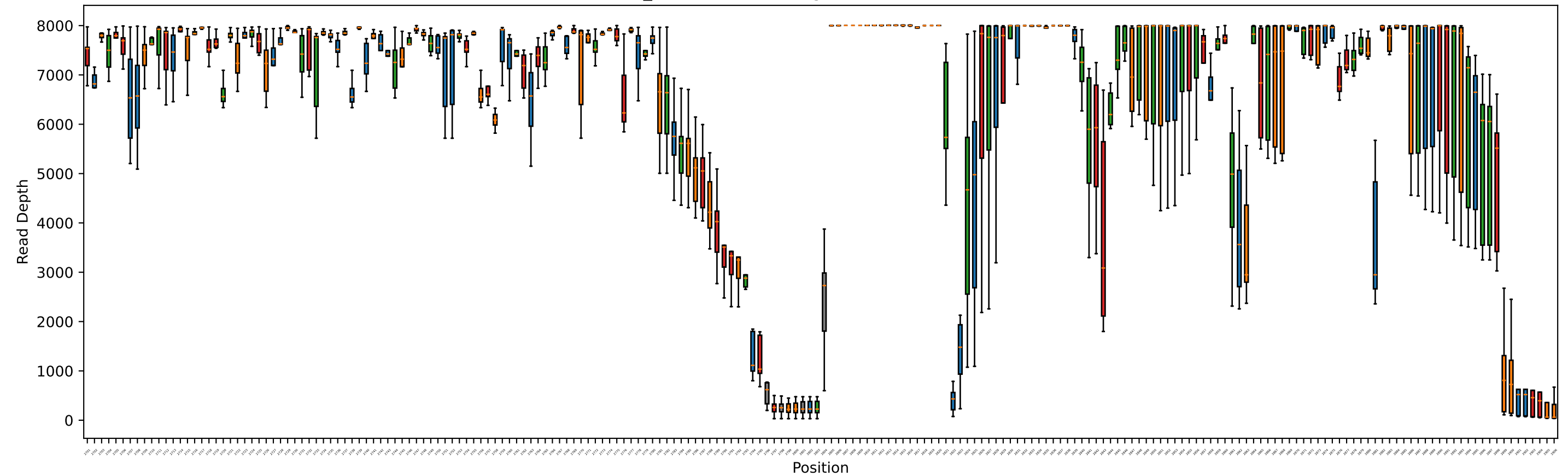
23S_consensus Coverage - Positions 2701-2906
