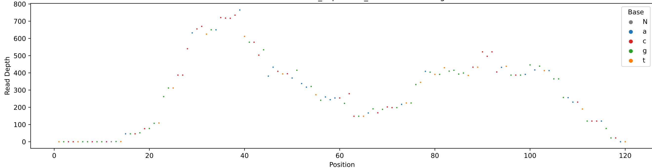
SRR10533473.sorted_depth - 5S_consensus Coverage
