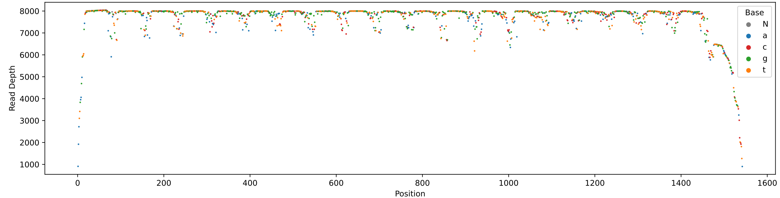
SRR11584025.sorted_depth - 16S_consensus Coverage
