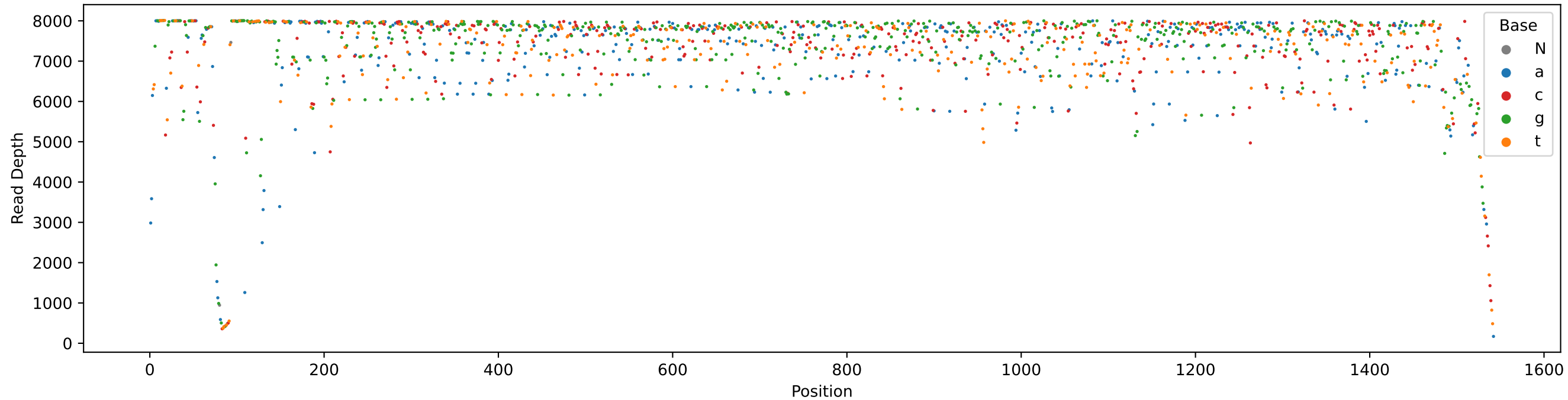
SRR11584028.sorted_depth - 16S_consensus Coverage
