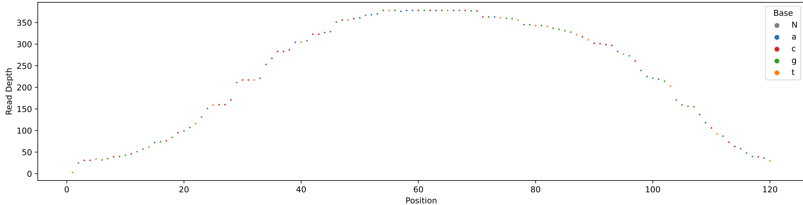
SRR11584025.sorted_depth - 5S_consensus Coverage
