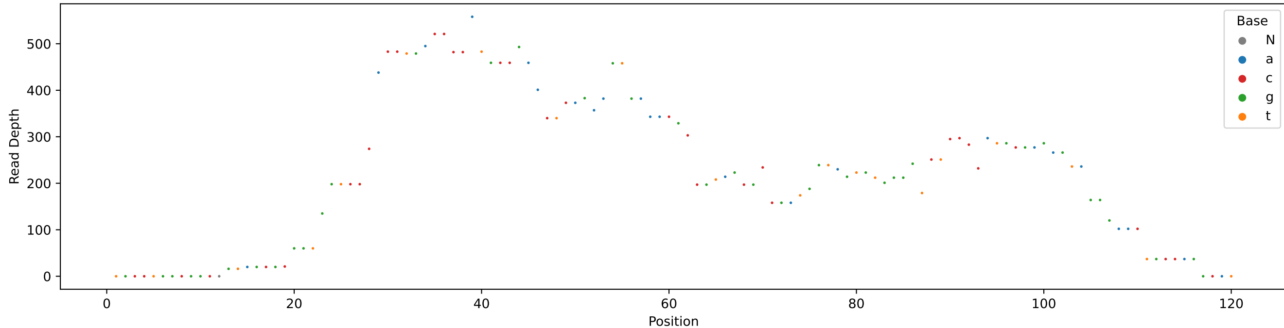
SRR10533474.sorted_depth - 5S_consensus Coverage
