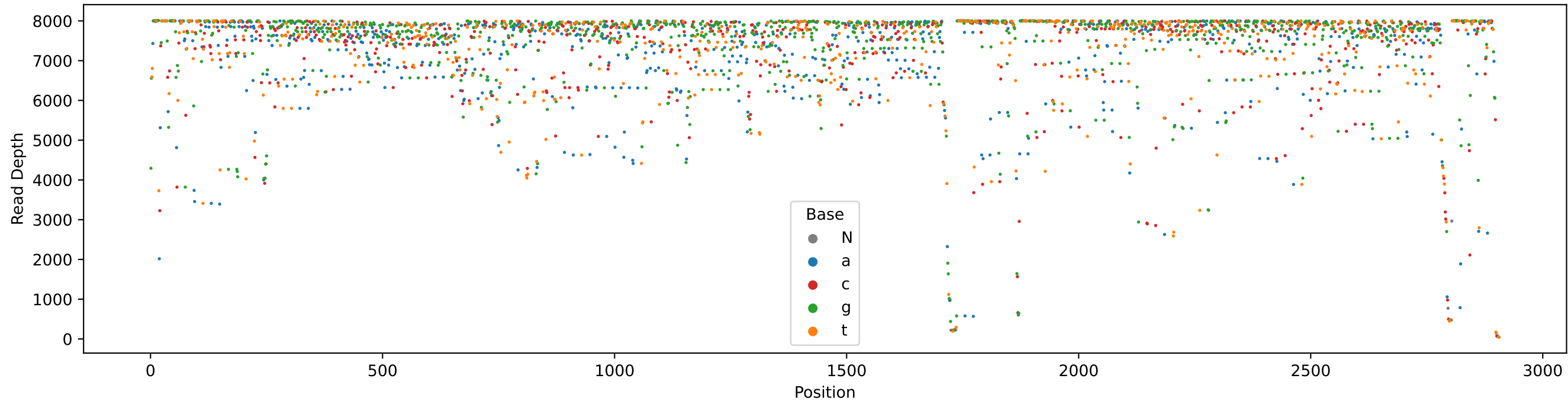
SRR11584028.sorted_depth - 23S_consensus Coverage
