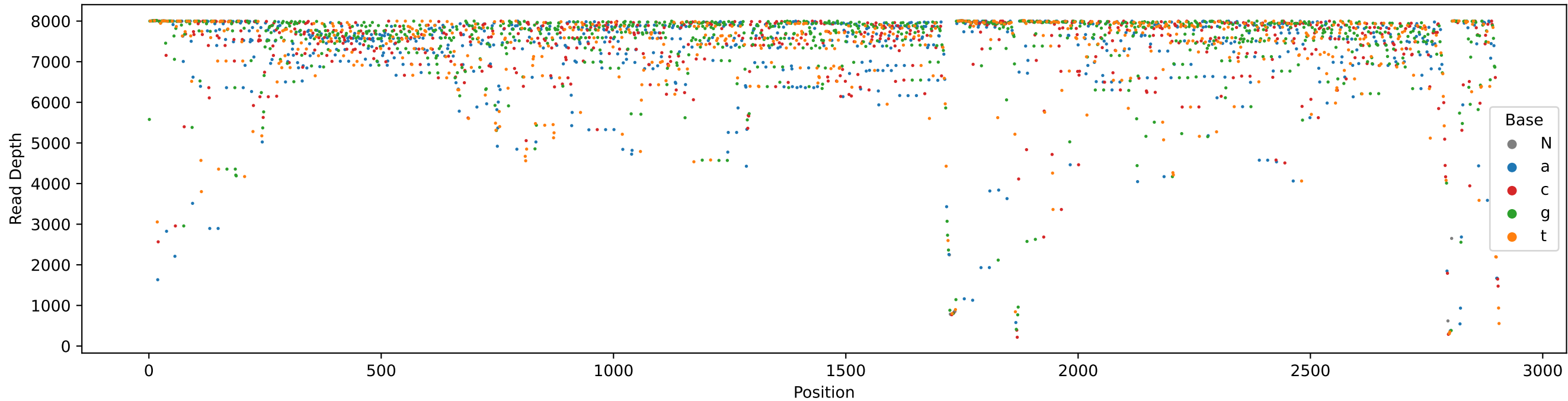
SRR10533475.sorted_depth - 23S_consensus Coverage
