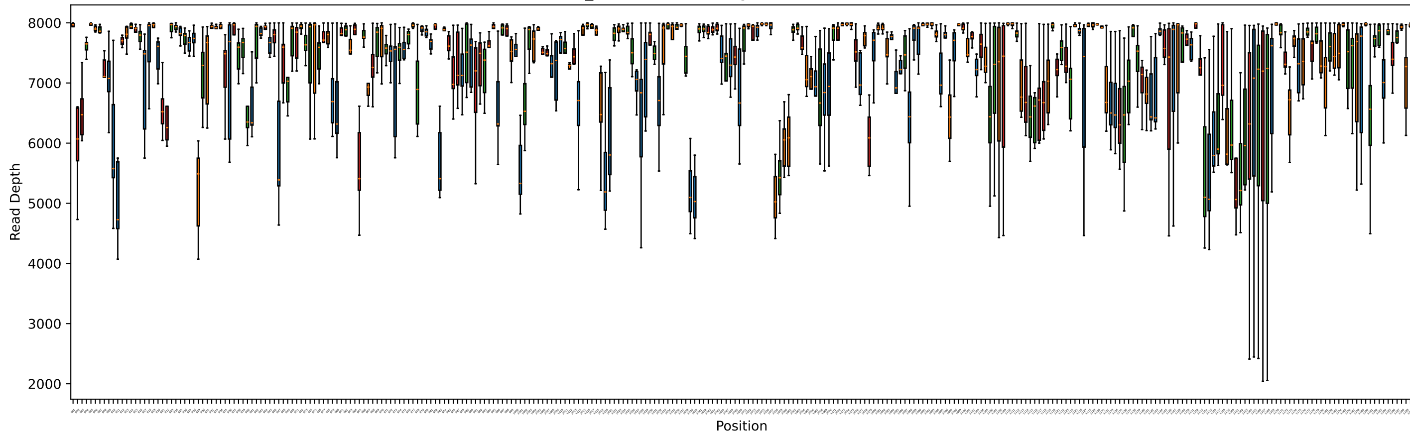
23S_consensus Coverage - Positions 901-1200
