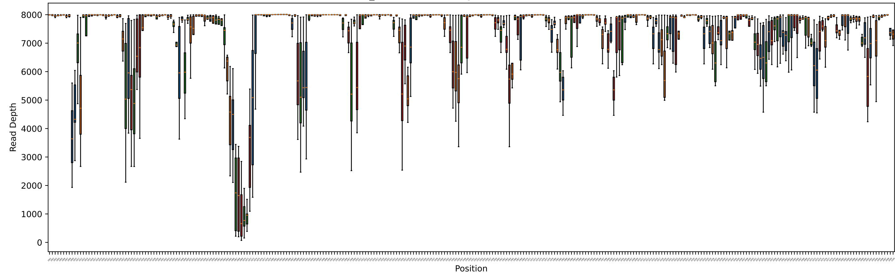
23S_consensus Coverage - Positions 1801-2100
