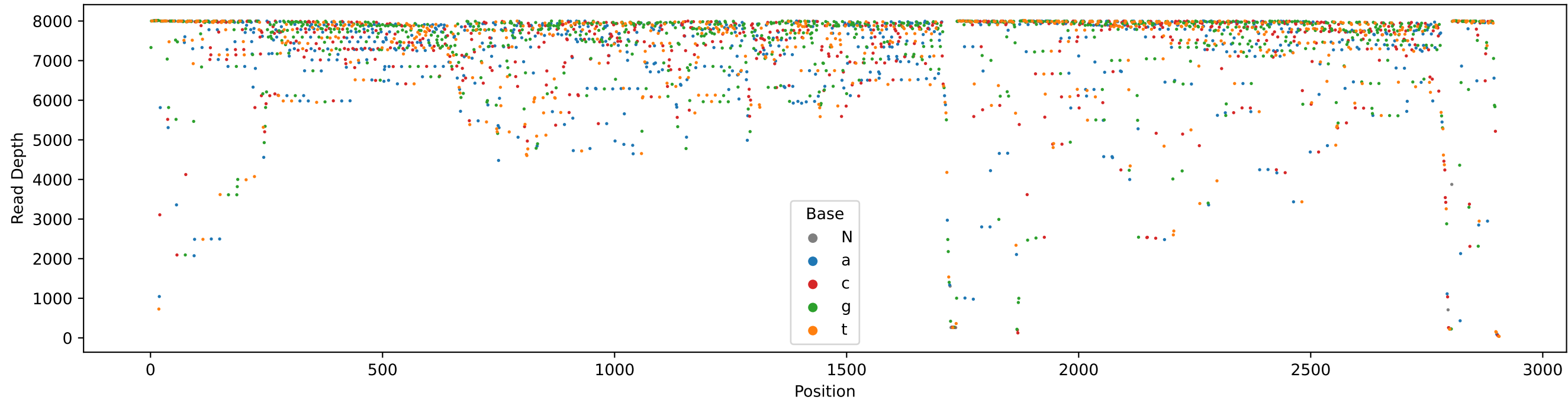
SRR10533476.sorted_depth - 23S_consensus Coverage
