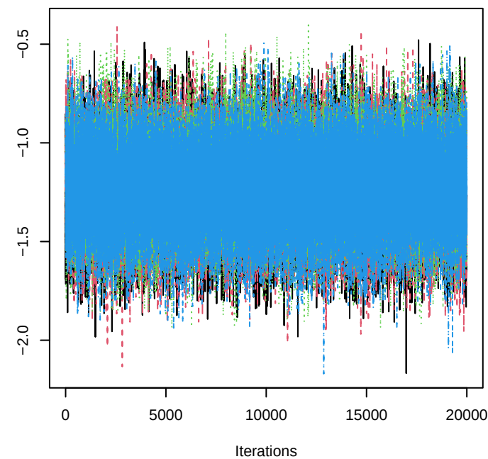
Trace of beta 400
