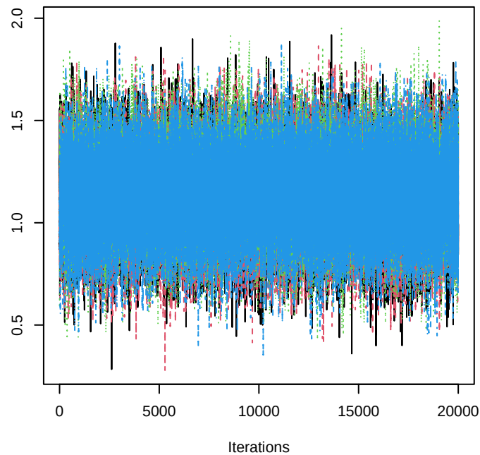
Trace of beta 660
