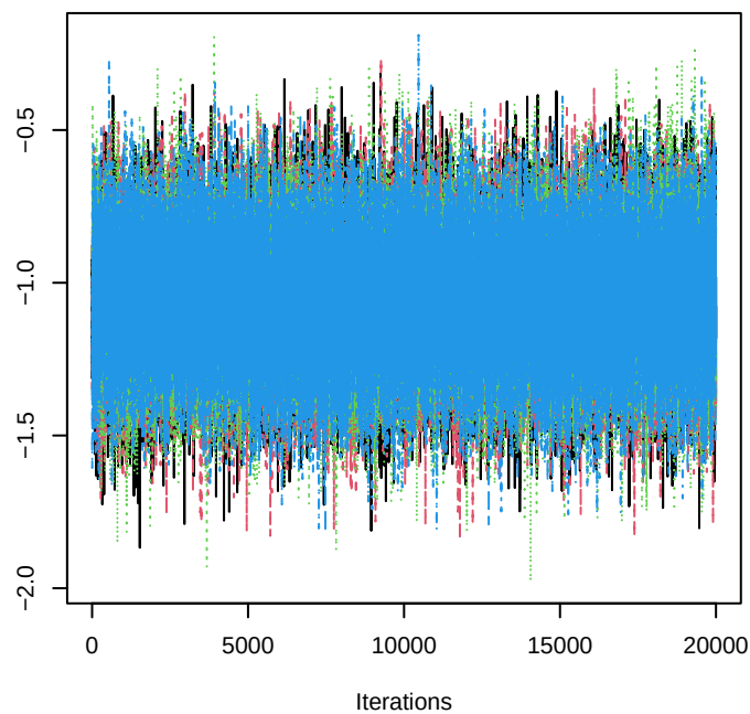
Trace of beta 700
