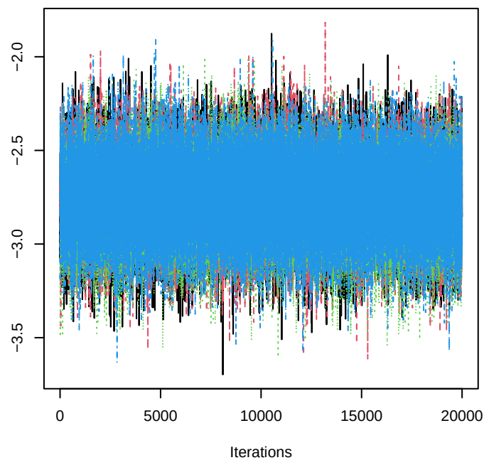
Trace of beta 380
