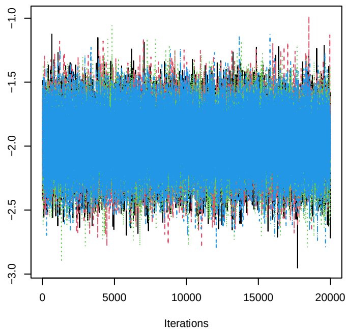
Trace of beta 240
