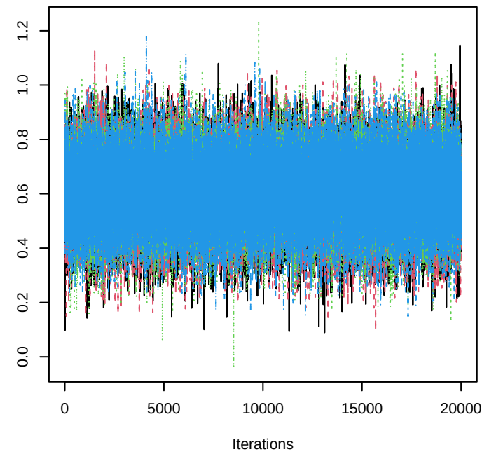
Trace of beta0
