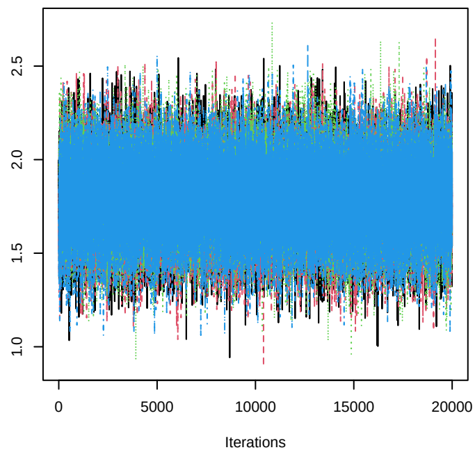
Trace of beta 260
