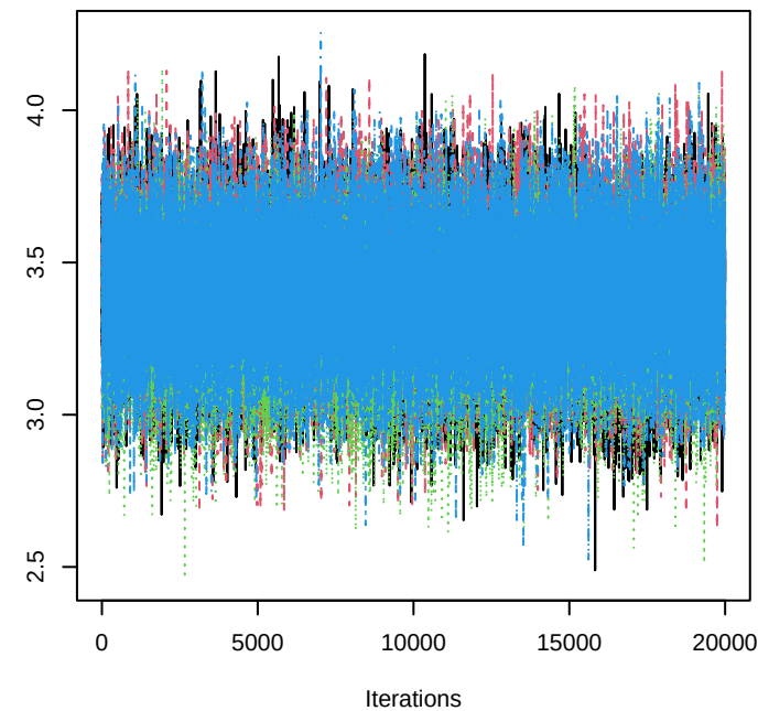
Trace of beta 680
