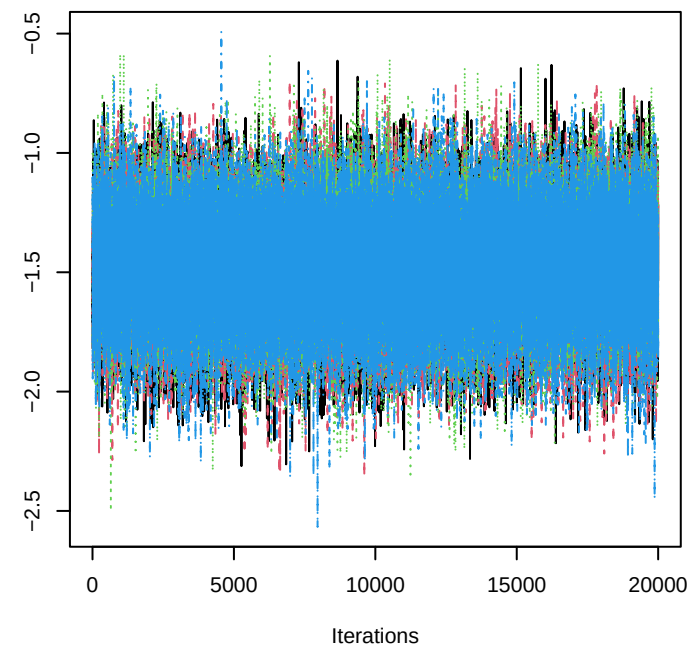
Trace of beta 620
