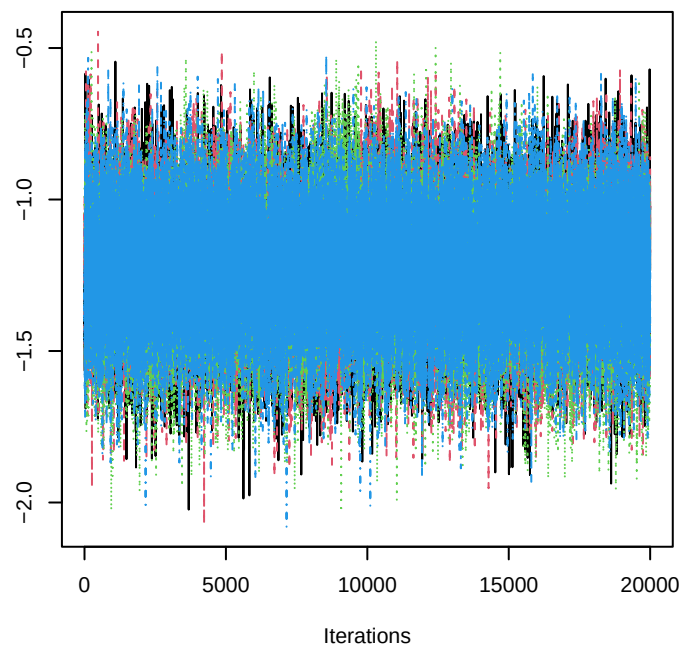
Trace of beta 780
