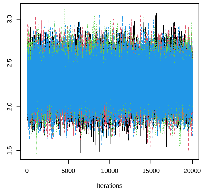
Trace of beta 740
