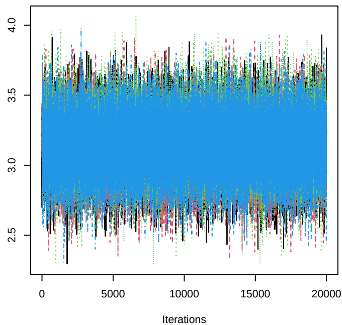
Trace of beta 580
