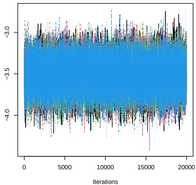
Trace of beta 320
