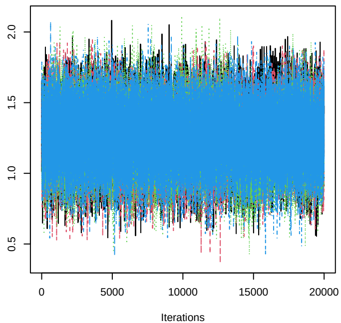
Trace of beta 760
