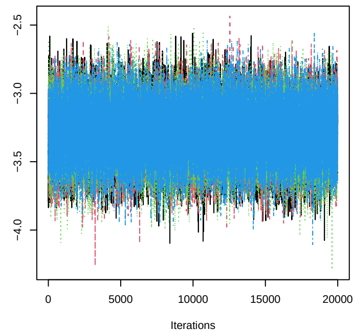
Trace of beta 340
