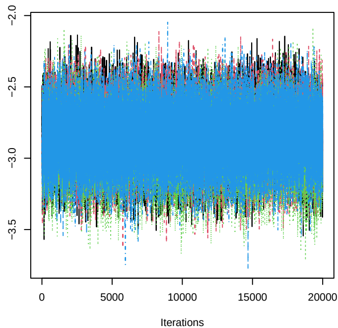
Trace of beta 600
