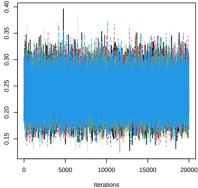
Trace of alpha
