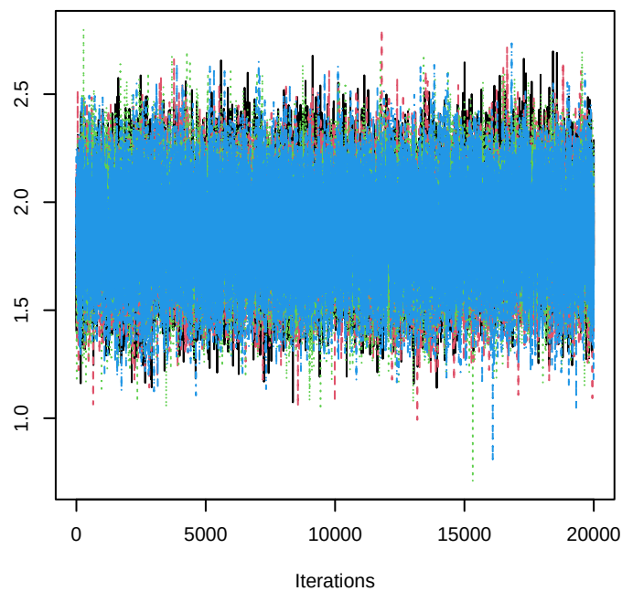
Trace of beta 300
