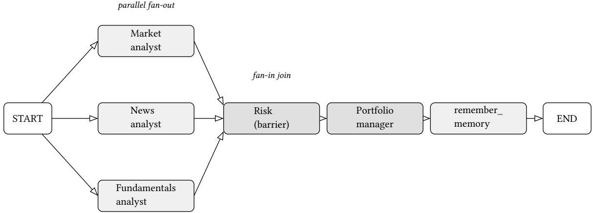
Figure 1: LEGACY LangGraph topology: START fans out to three parallel analysts, each running an isolated tool sub-loop; the barrier risk node joins them once all reports exist; the portfolio manager emits the typed decision; and remember_memory persists it before END . Each analyst also has a hidden ToolNode self-loop (omitted for clarity).
