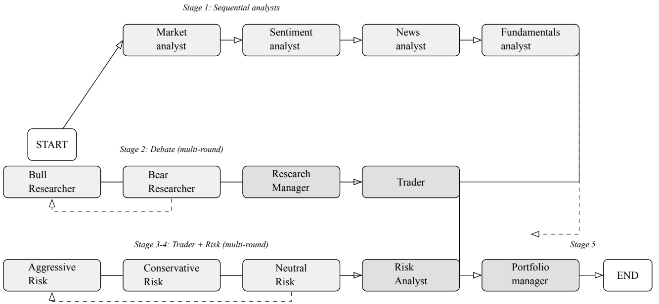
Figure 1: LangGraph pipeline topology: four sequential analysts (Stage 1) feed into a multi-round bull/bear debate (Stage 2), a Research Manager and Trader (Stage 3), a three-way risk discussion (Stage 4), and the Portfolio Manager (Stage 5). Dashed lines denote debate loops; each analyst has a hidden ToolNode self-loop and message-clearing node (omitted for clarity).
