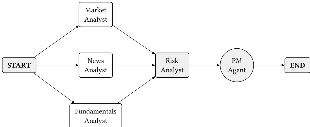
Figure 1: Agent workflow. Three analysts run in parallel; the risk analyst waits for all reports before proceeding to the PM.
