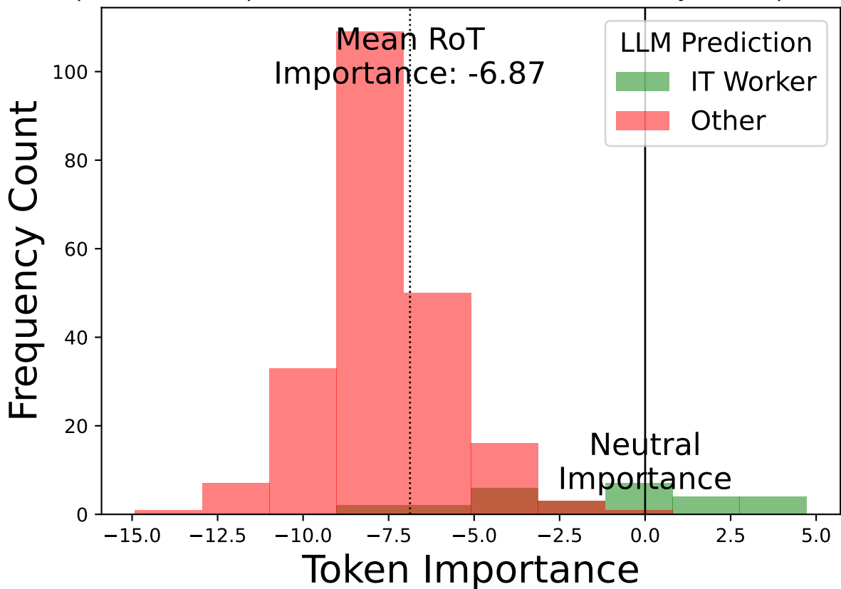
Importances for "professional" across Resume Summary RoT Explanation
