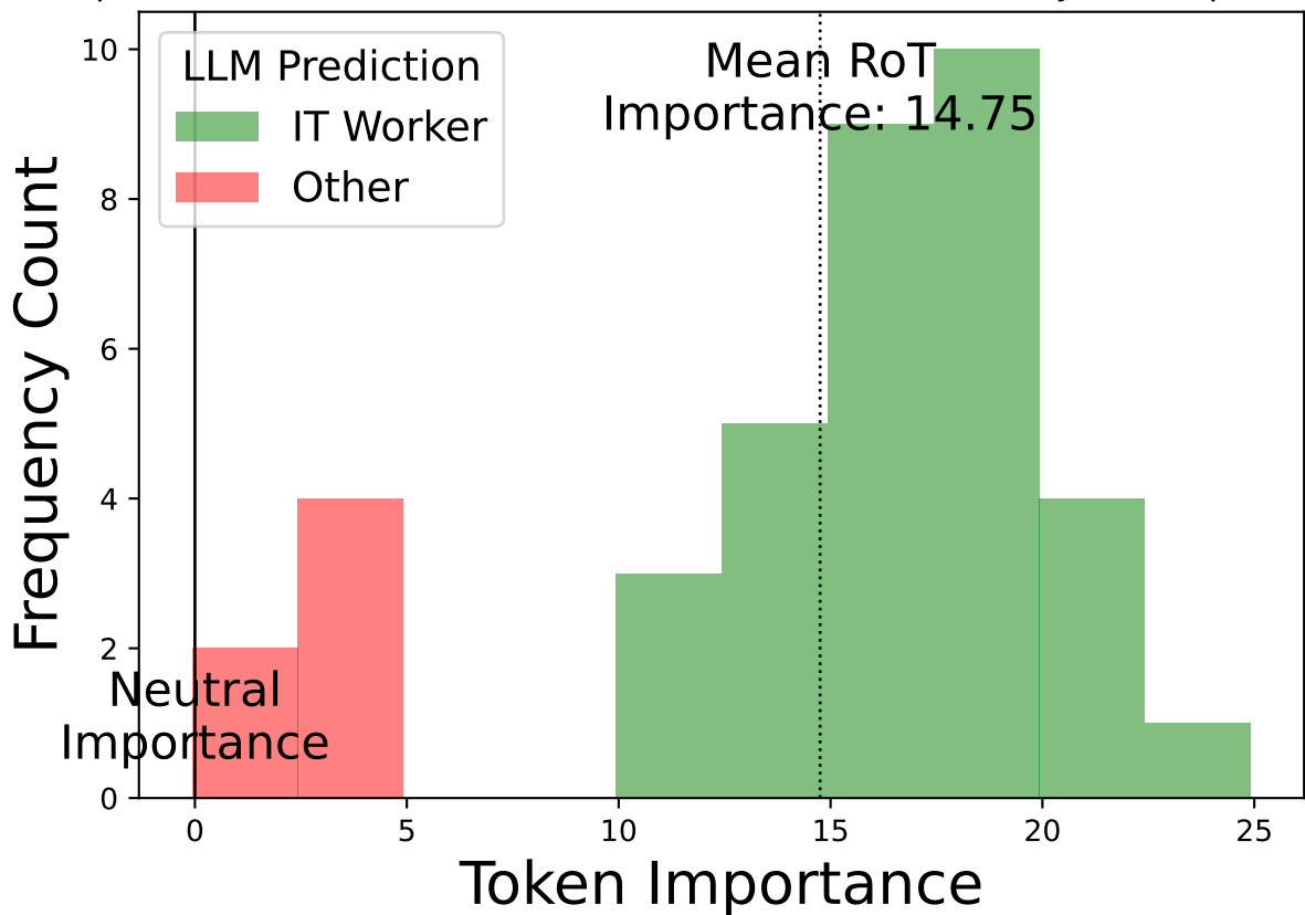
Importances for "infrastructure" across Resume Summary RoT Explanation
