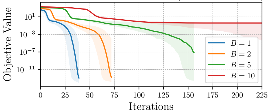
Convergence Comparison (median \pm IQR)
