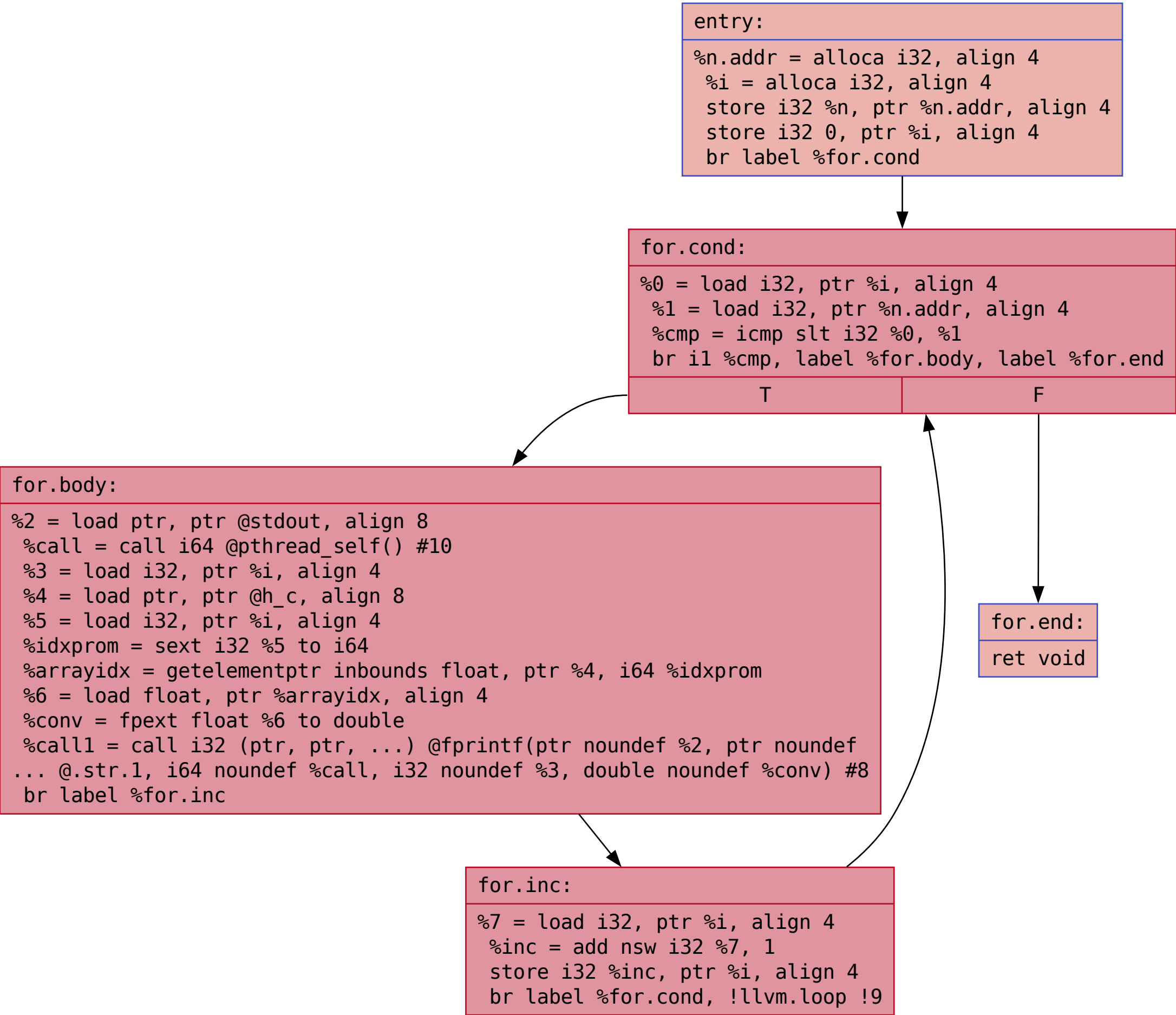
CFG for 'print_array' function
