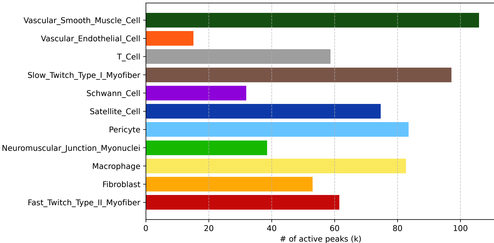
Active peaks in Muscle_Quadriceps (N=280991) (mean = 64k median = 62k)
