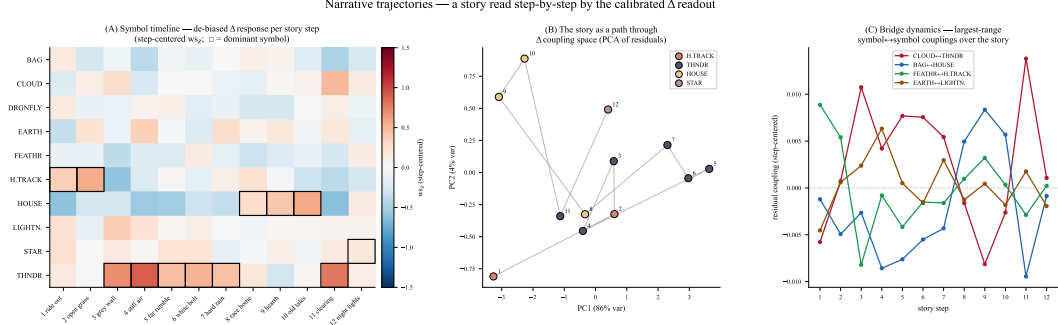
Figure 7: Narrative trajectories. A twelve-step story read by the calibrated \Delta readout. (A) symbol timeline: de-biased per-symbol response per step, the dominant symbol boxed, the hot spot following the arc. (B) the story as a connected path through coupling space (PCA of per-step residual recouplings). (C) dynamics of the four highest-range symbol–symbol couplings. The story is a trajectory, not a point.
