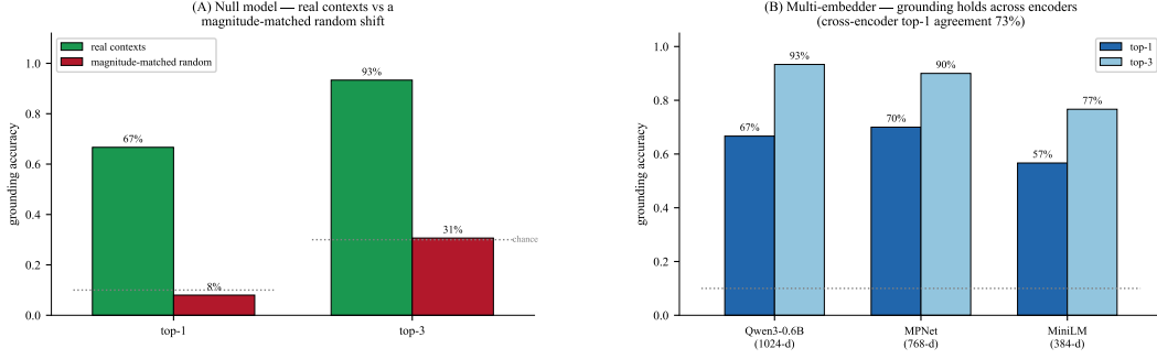
Figure 10: Robustness. (A) Null model: real contexts recover the intended symbol far above a magnitude-matched random shift (top-1 67% vs 8%; top-3 93% vs 31%; chance 10/30%), so the re-couplings are structured signal, not a by-product of shift magnitude. (B) Multi-embedder: grounding holds across three unrelated encoders (Qwen3, MPNet, MiniLM), with 73% cross-encoder agreement on the assigned symbol: the readout is not an artifact of one model’s geometry.
