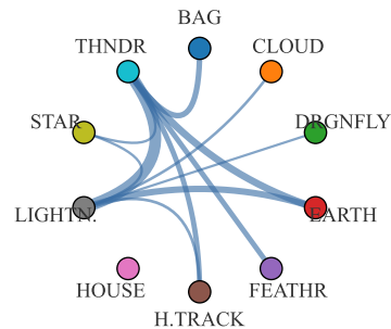
(B1) thunder: \Delta subgraph (symbols)
