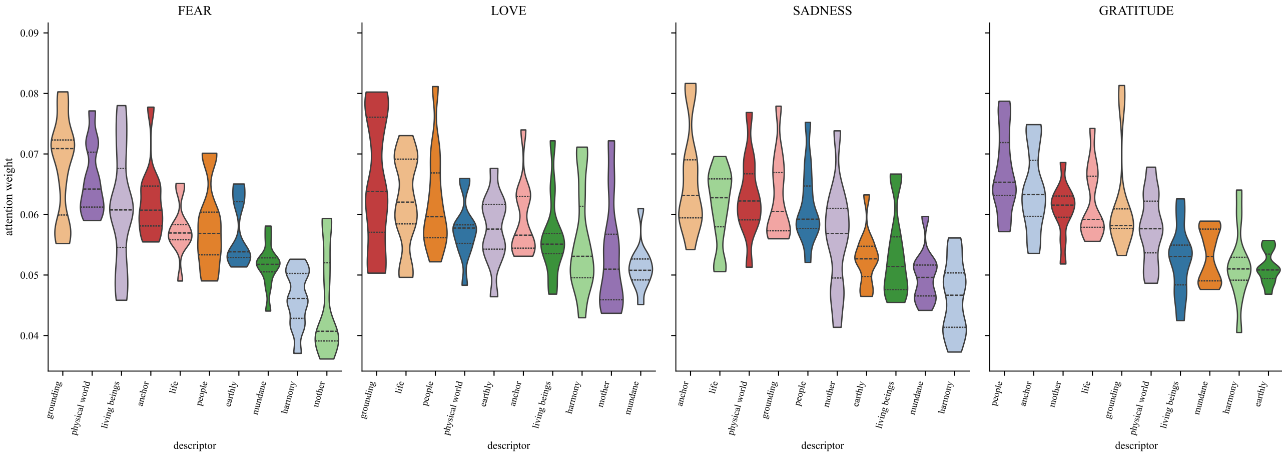
EARTH — descriptor attention per thematic context (top-10, sorted within each panel; \tau=0.2 )
