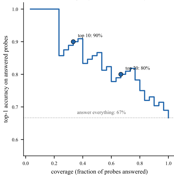
(B) High-margin probes are the confident ones; answering only those raises accuracy
