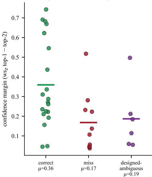
(A) The margin separates settled from open readings (AUC 0.78); ambiguous phrases land with the open ones
