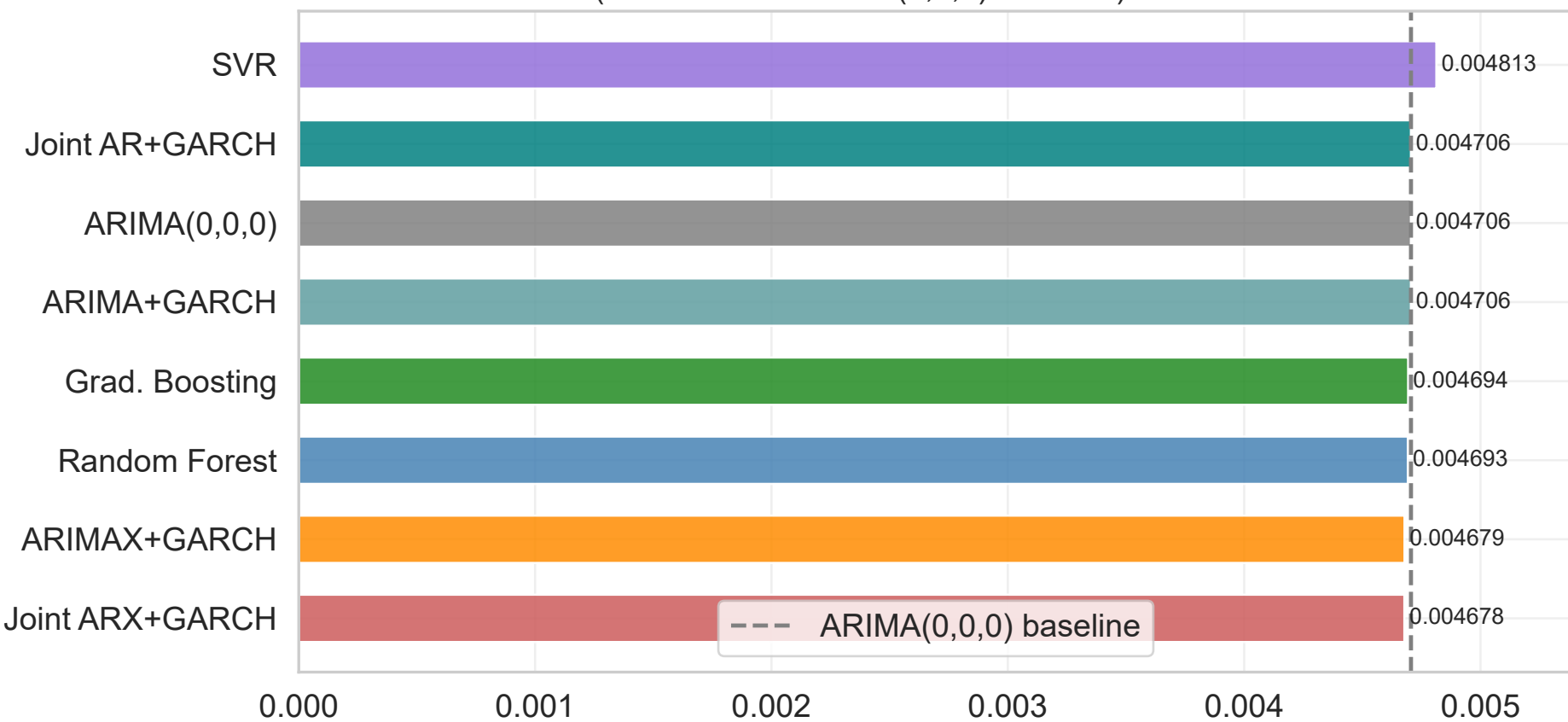
DXY — OOS RMSE (all models vs ARIMA(0,0,0) baseline)
