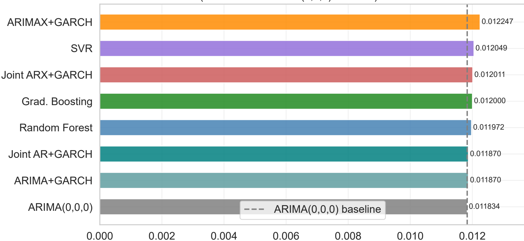
EEM — OOS RMSE (all models vs ARIMA(0,0,0) baseline)
