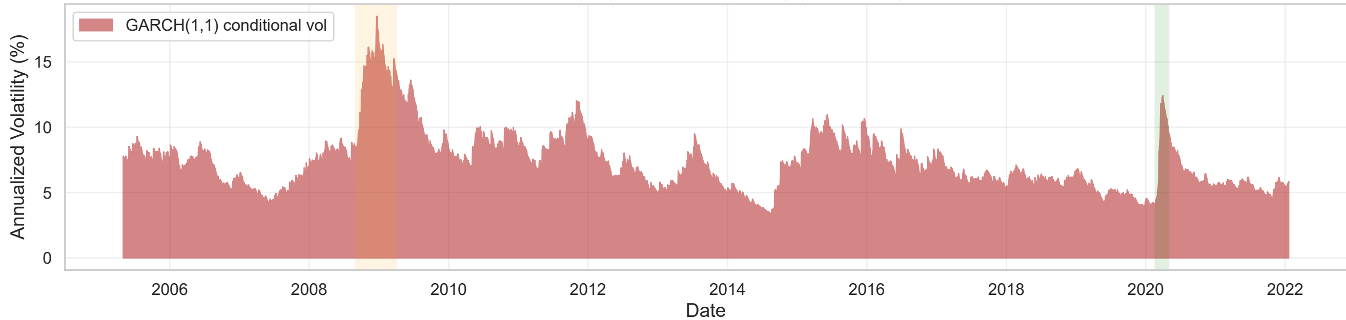
GARCH(1,1) Conditional Volatility (Annualized)
