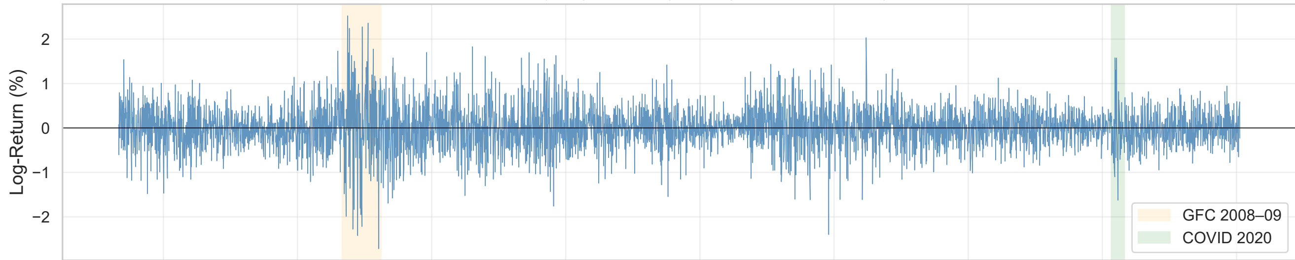
DXY Daily Log-Returns (Training Set: 2005 – 2022)
