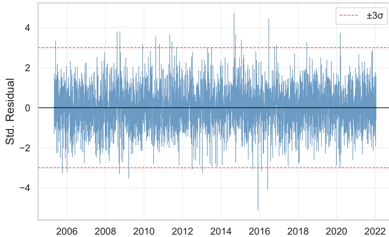
Standardized Residuals Over Time
