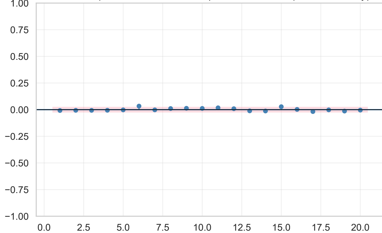
ACF of Squared Std. Residuals (flat = GARCH captured volatility)
