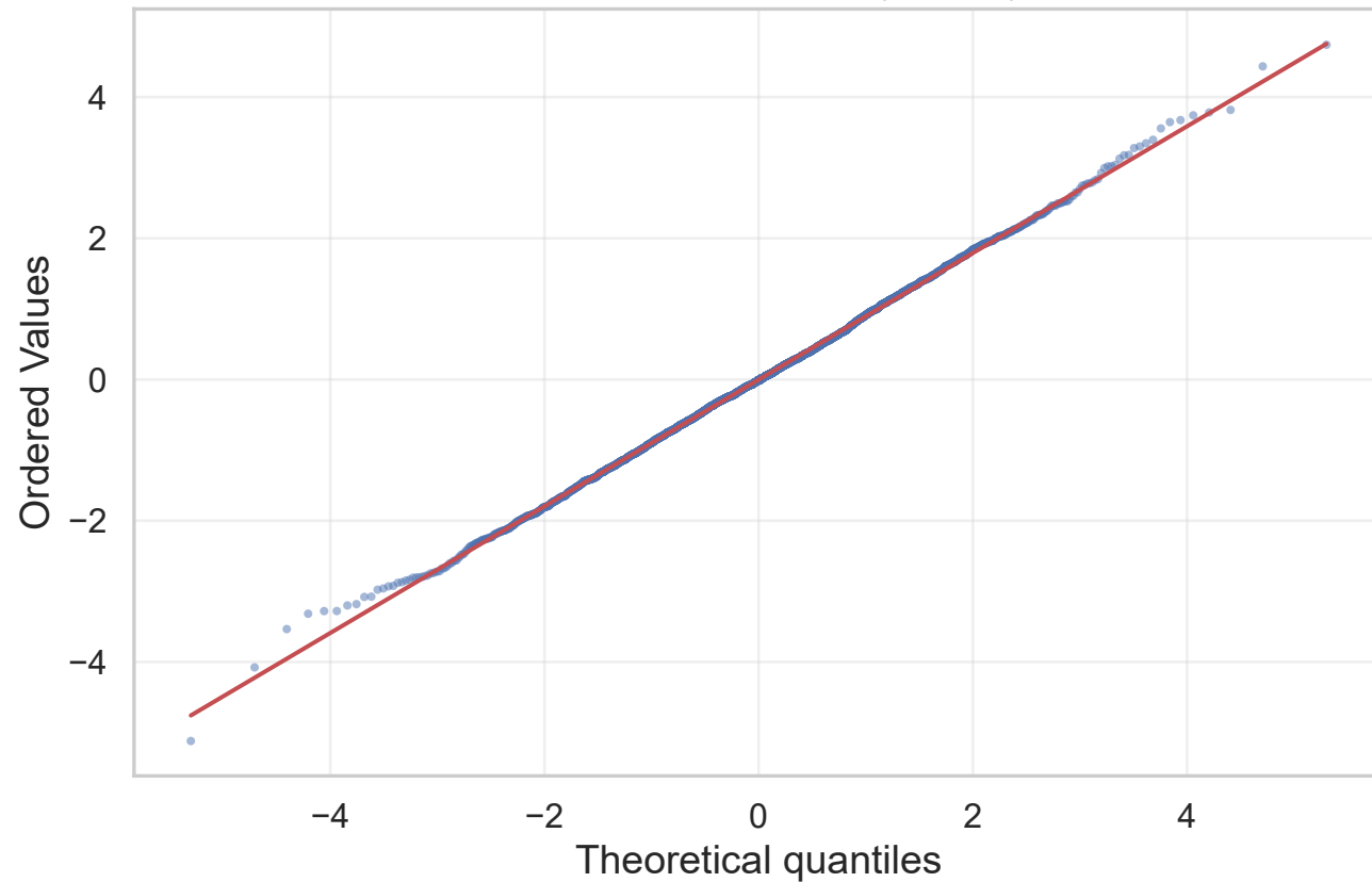
QQ-Plot vs Student-t ( \nu=10.2 )
