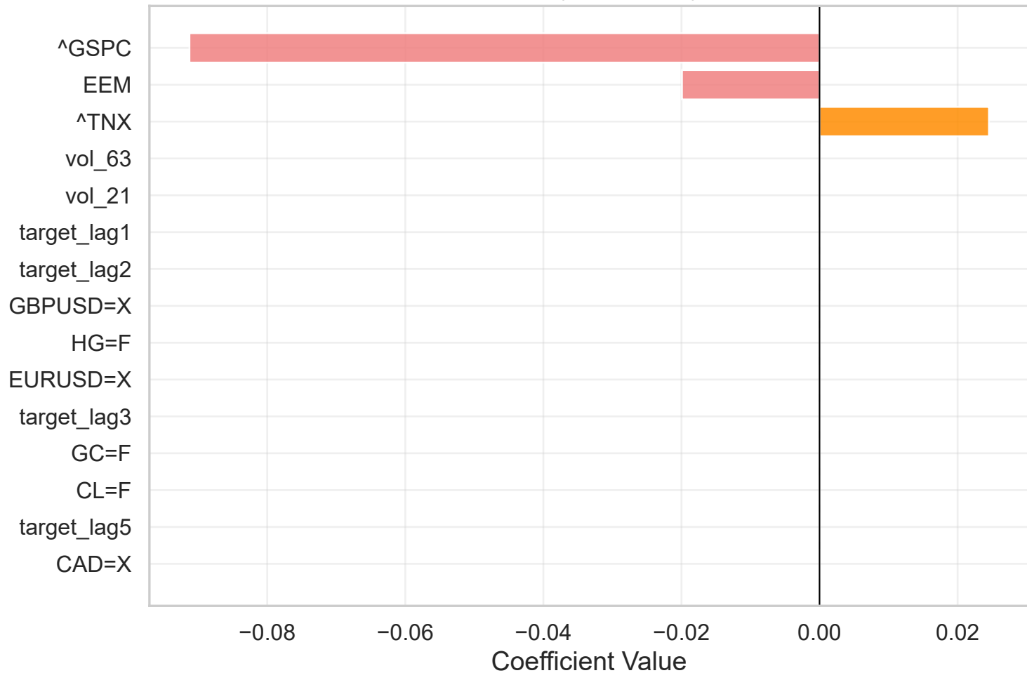
Lasso ( \alpha = 0.0231 )
