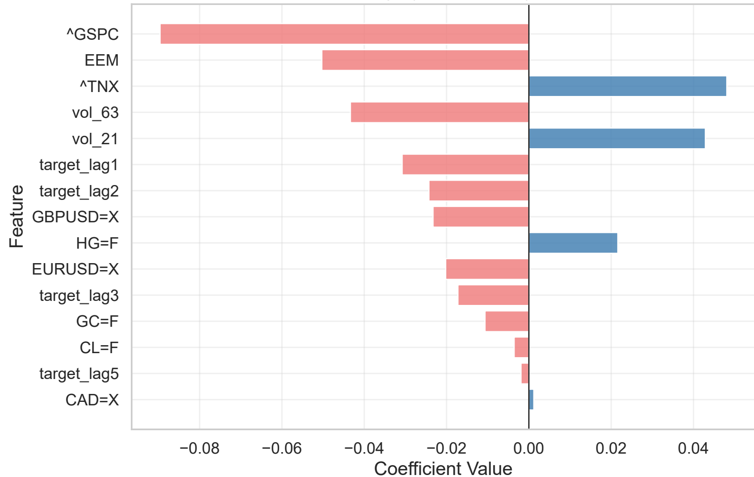
Ridge ( \alpha = 657.9332 )
