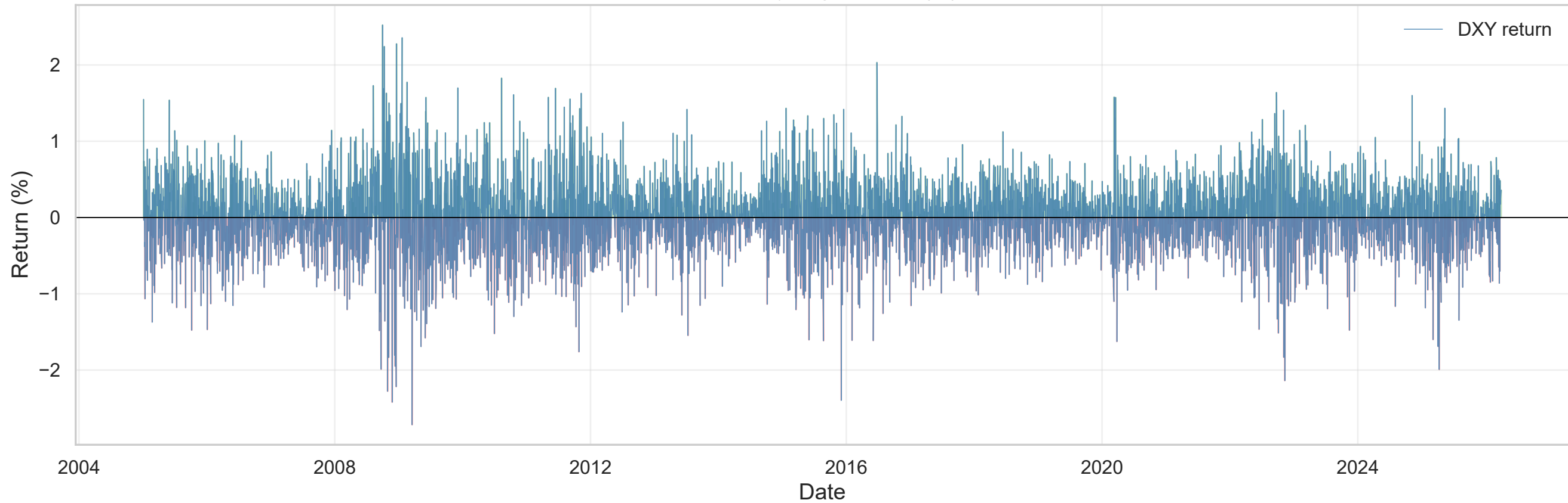
DXY Daily Log-Returns (%)
