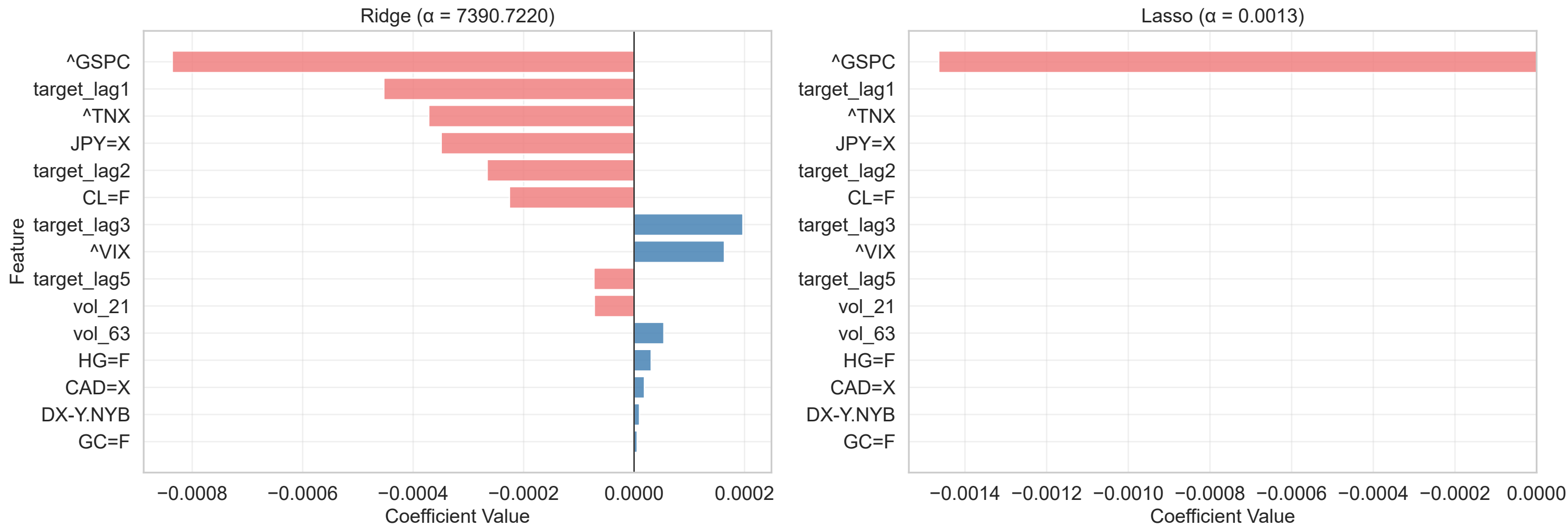
Ridge vs Lasso Feature Weights — 15-Feature Set (blue=positive, red=negative)
