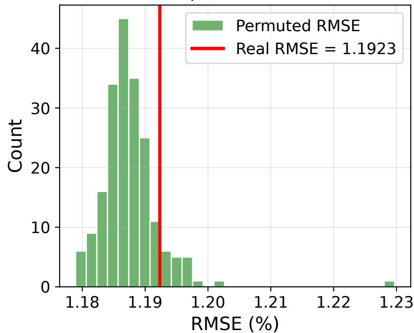
Grad. Boosting p = 0.905
