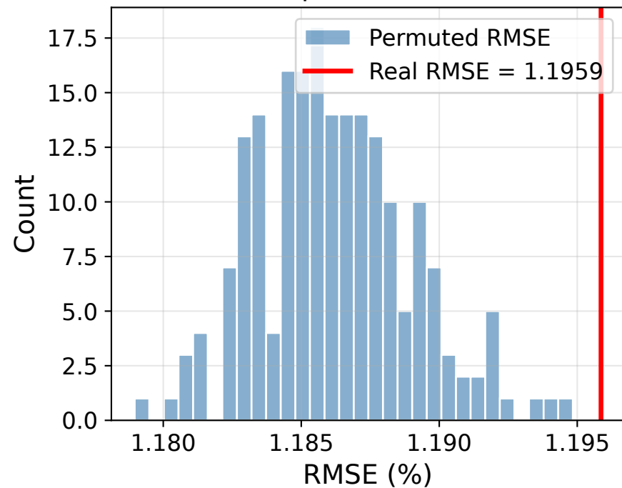
Random Forest p = 1.000
