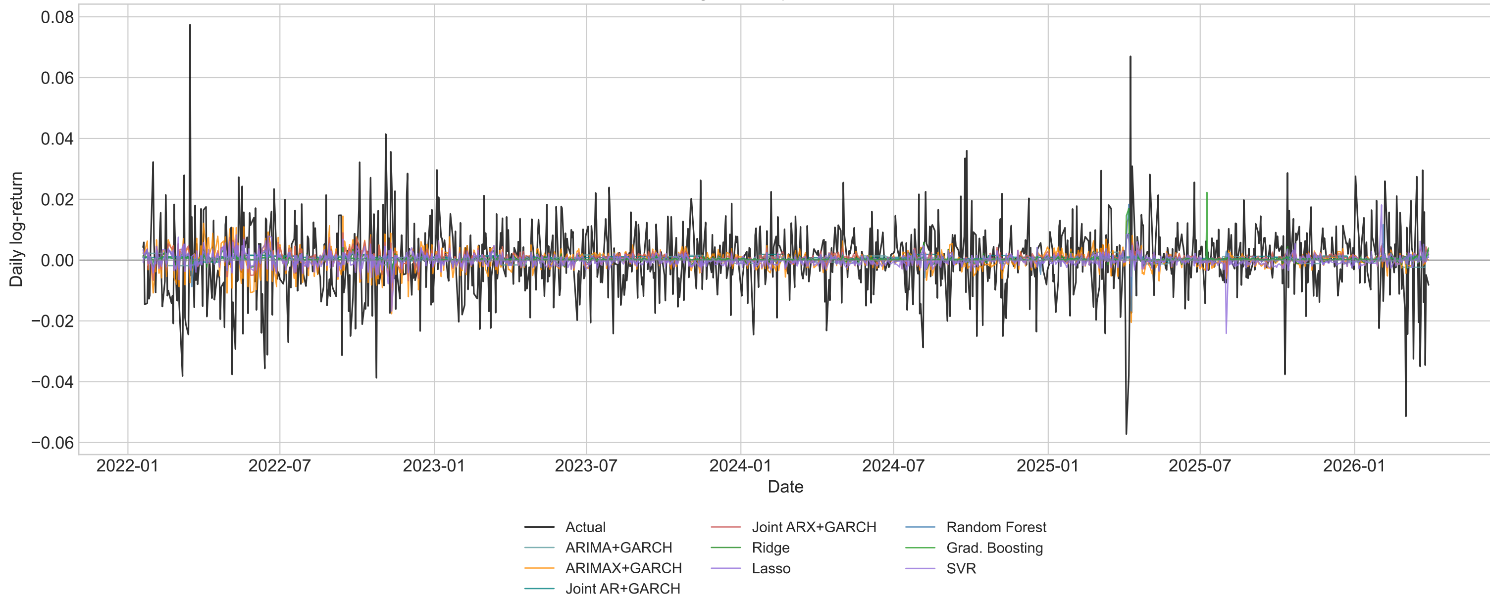
EEM — rolling one-step-ahead OOS forecasts
