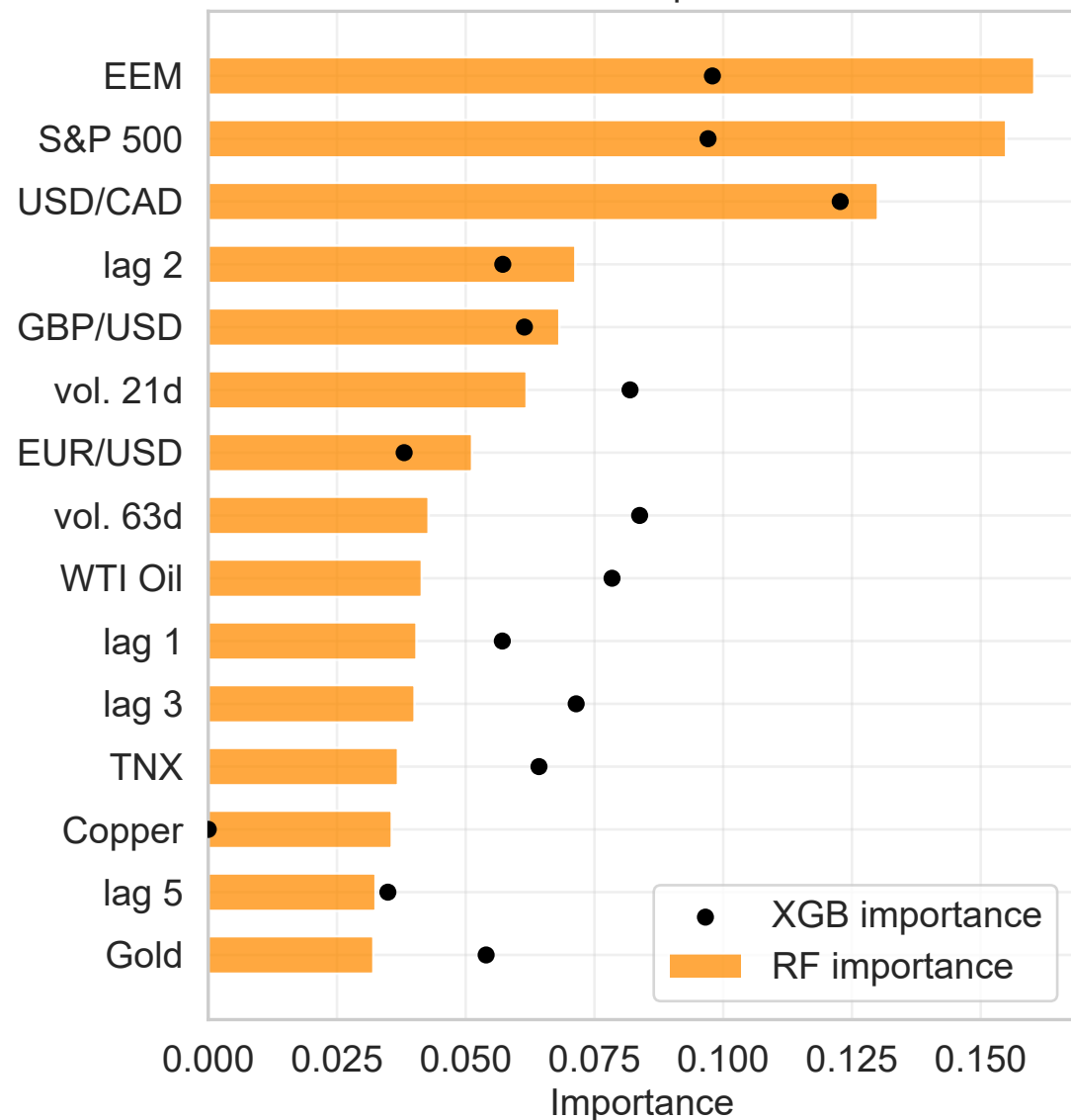
DXY — RF / XGB feature importance
