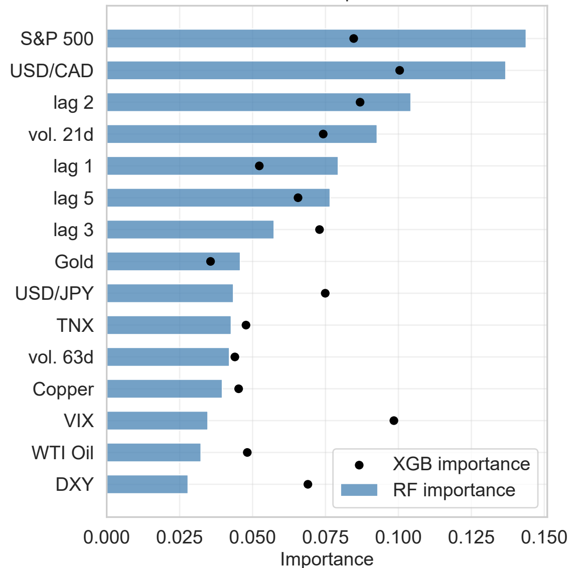
EEM — RF / XGB feature importance
