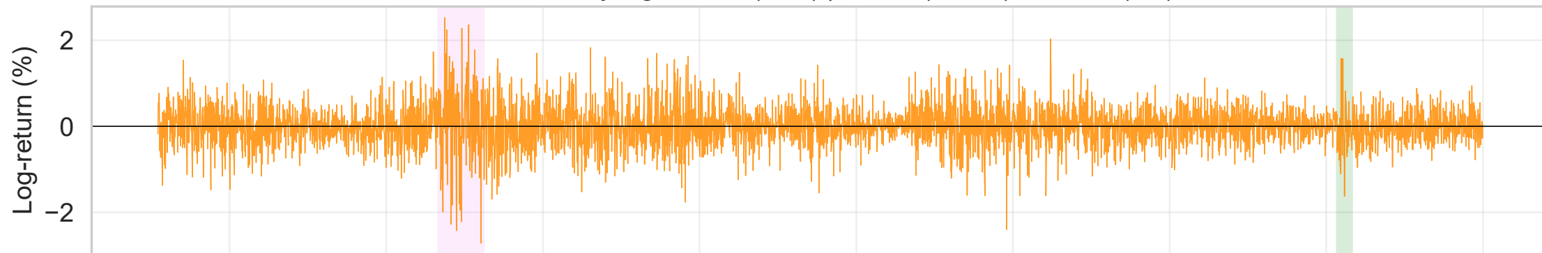
DXY — daily log-returns (train) | ARIMA(0, 0, 0)+GARCH(1,1)
