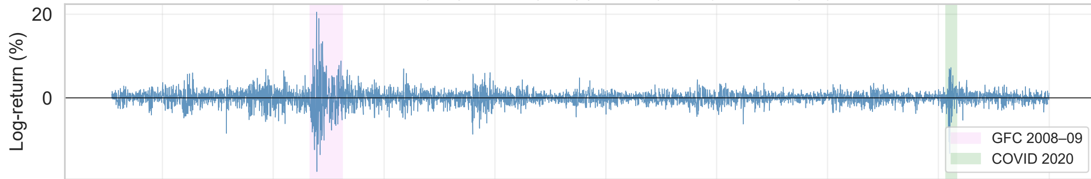
EEM — daily log-returns (train) | ARIMA(2, 0, 1)+GARCH(1,1)
