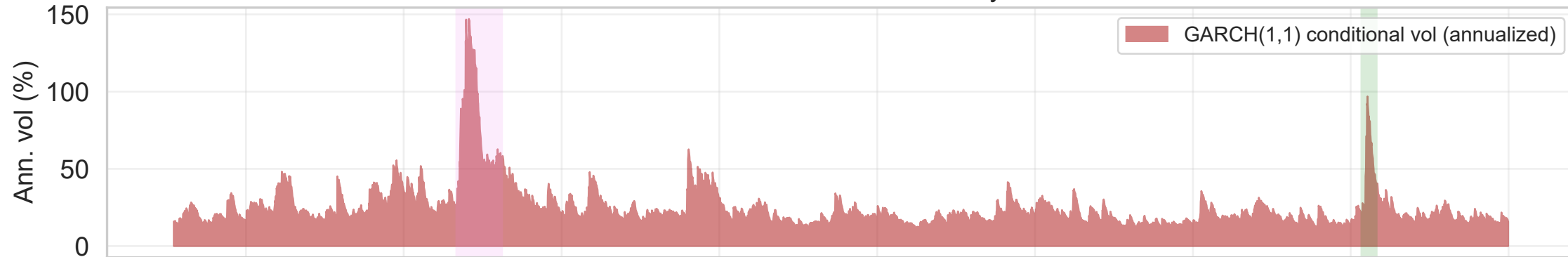
EEM — conditional volatility
