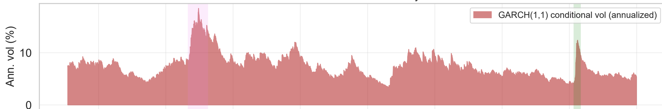
DXY — conditional volatility
