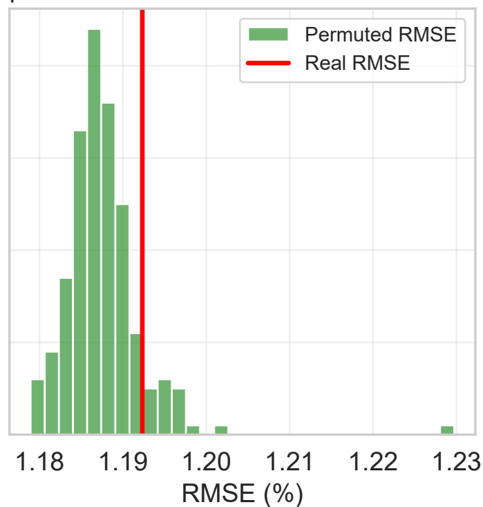
EEM - Grad. Boosting p = 0.905
