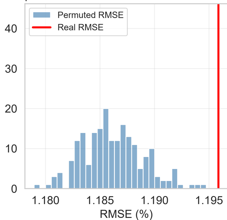
EEM - Random Forest p = 1.000
