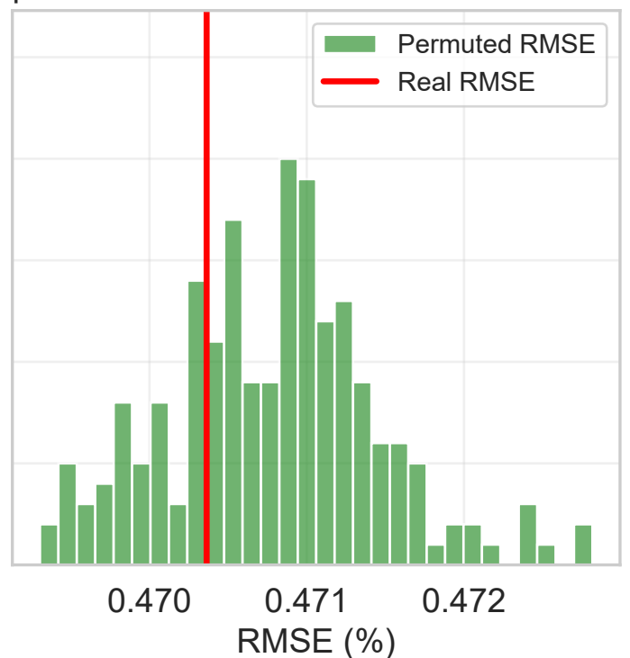
DXY - Grad. Boosting p = 0.270
