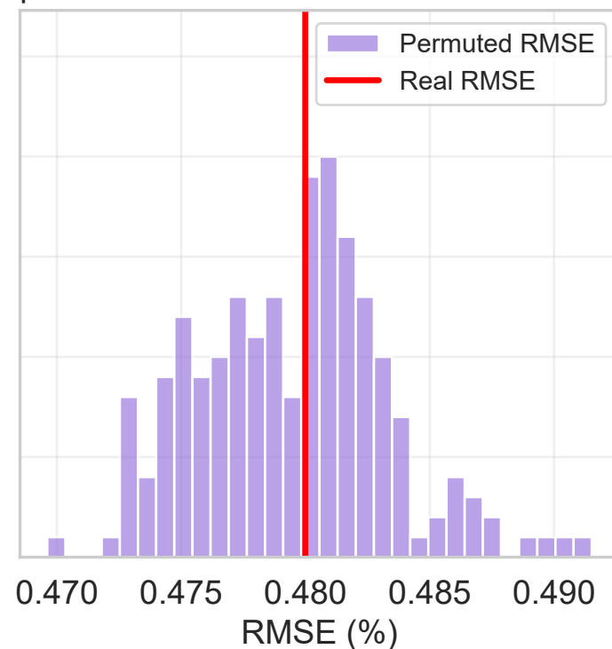
DXY - SVR p = 0.510
