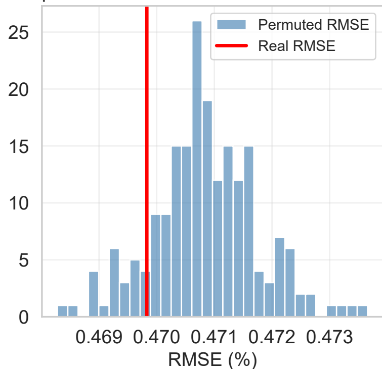
DXY - Random Forest p = 0.120
