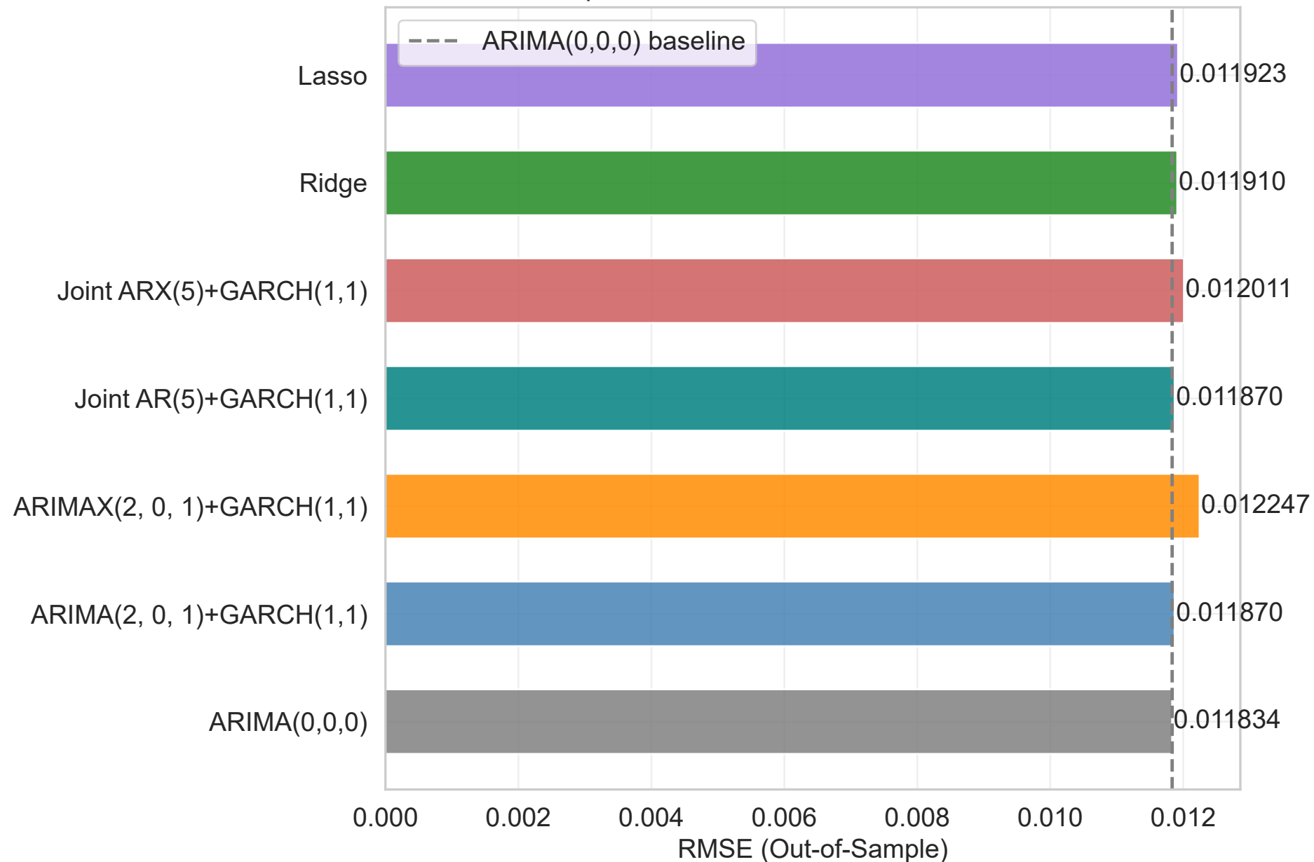
Out-of-Sample RMSE — All Models vs Random Walk Baseline
