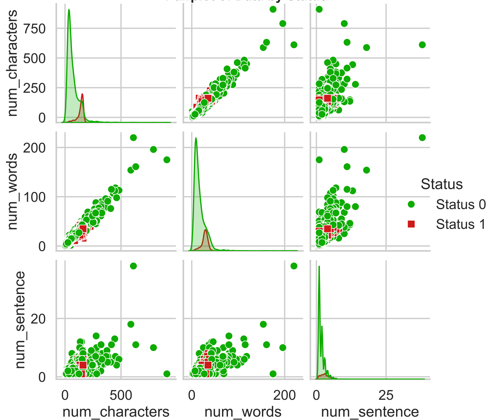
Pairplot of Data by Status
