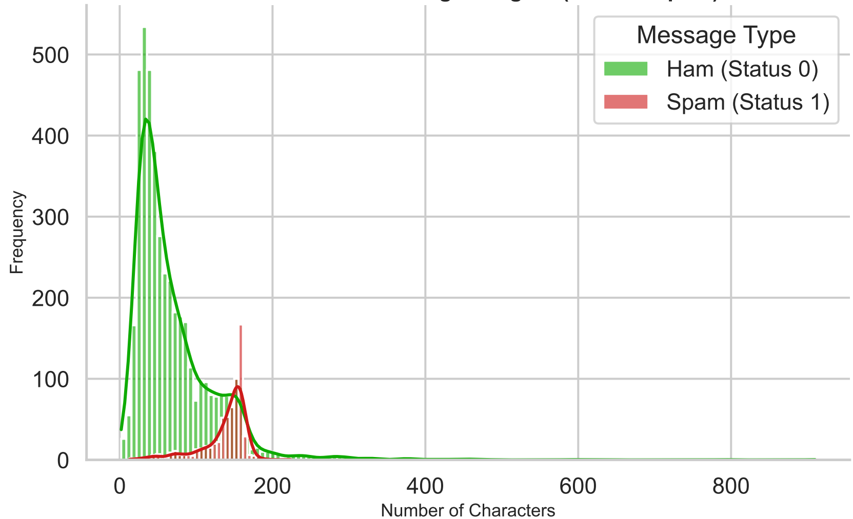
Distribution of Message Lengths (Ham vs Spam)
