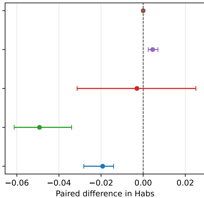
order reversal
