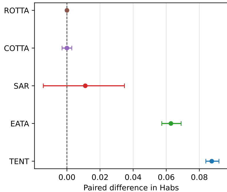
additional shift
