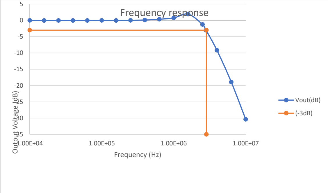
Op-amp frequency response
