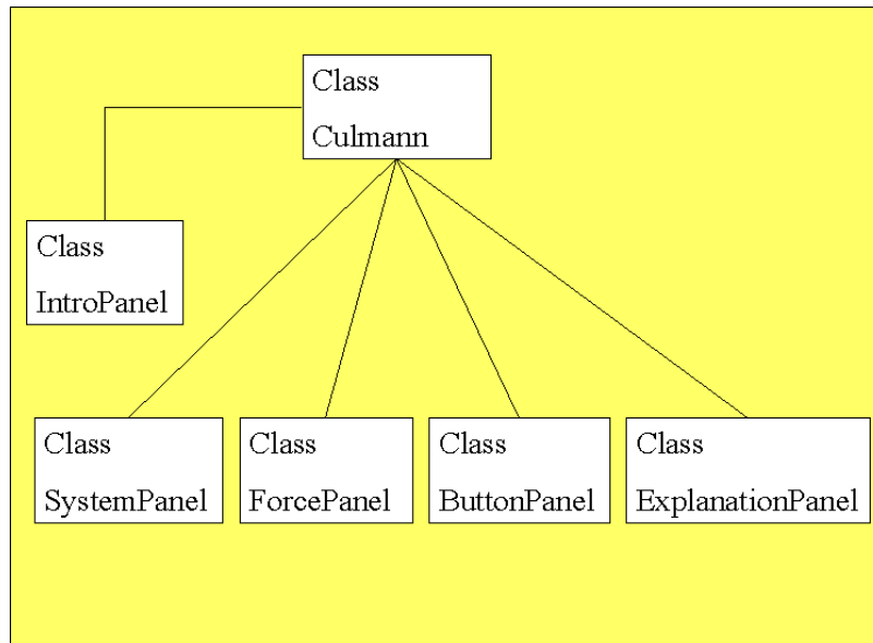
Figure 0-4: Class Diagram of the Culmann applet
