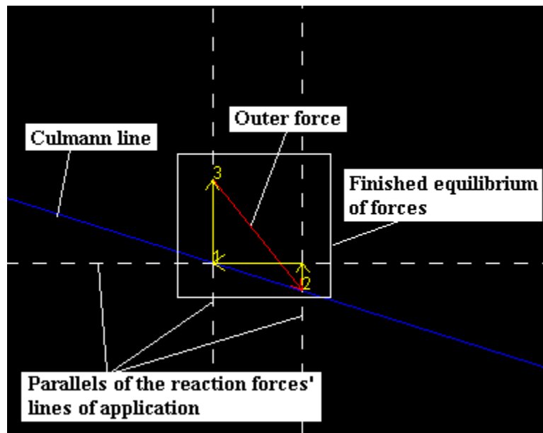
Figure 0-3: The Force Plan of the Culmann Method
