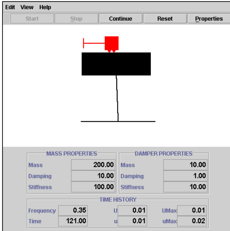
Figure 0-4: The Tuned Mass Damper applet
