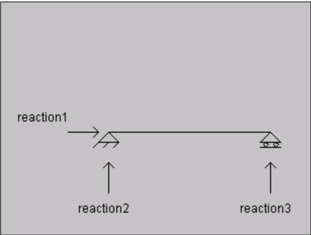
Figure 0-1: Example of a statically determinate system
