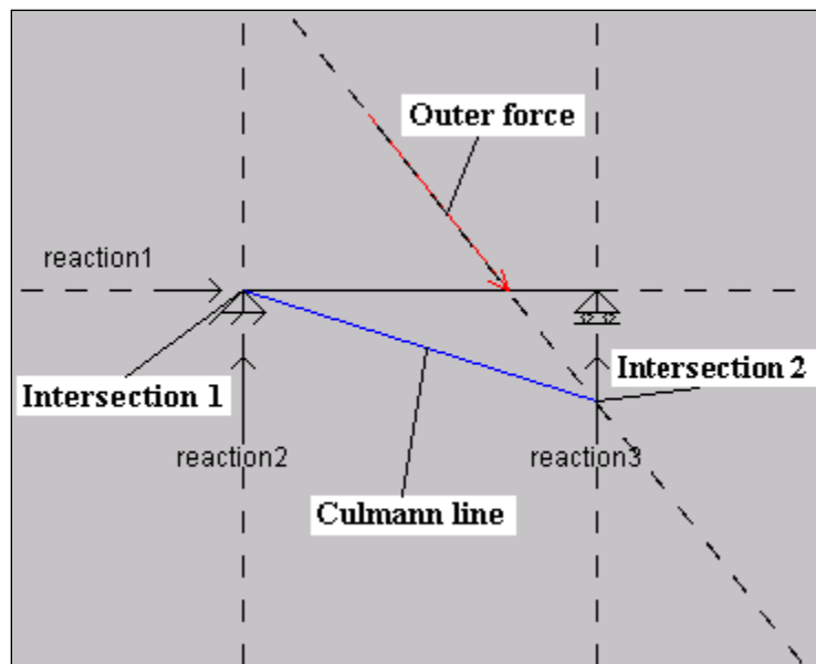
Figure 0-2: The Layout Plan of the Culmann Method
