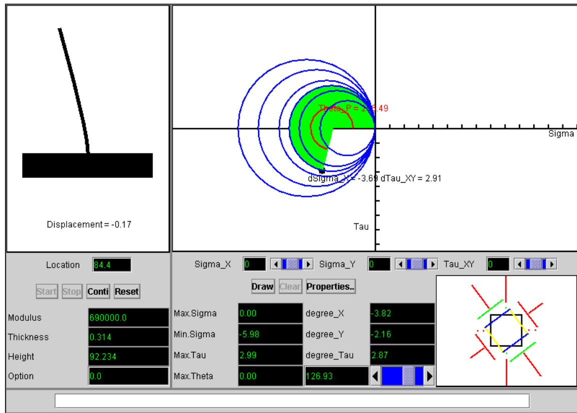
Figure 0-10: Real-Time Mohr's Circle applet
