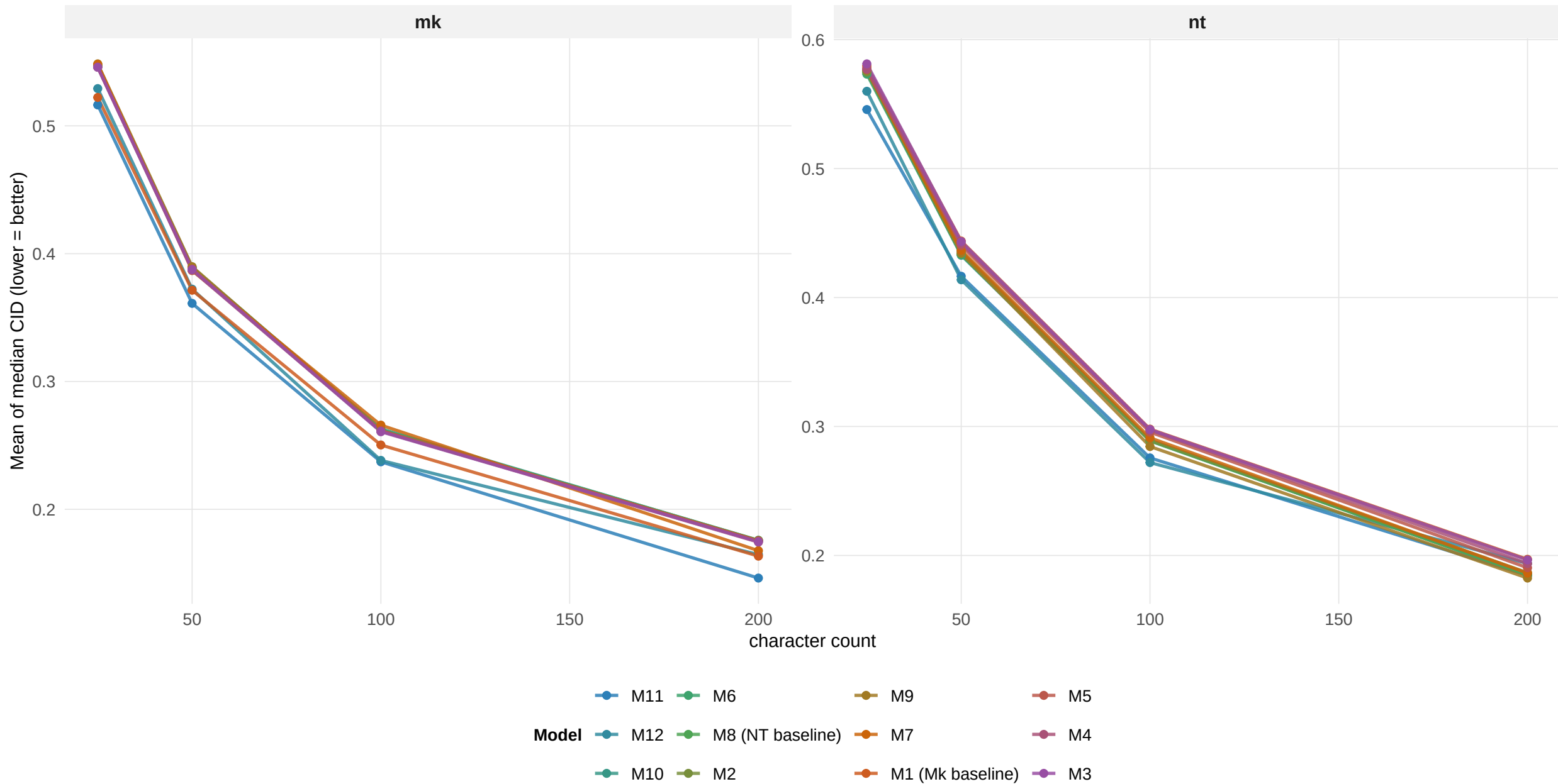
Effect of character count on tree accuracy, by model
