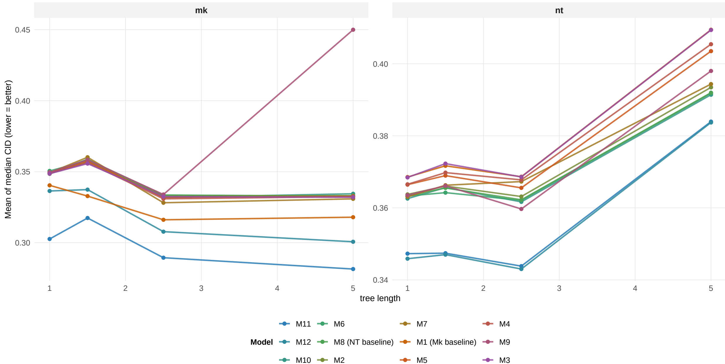
Effect of tree length on tree accuracy, by model
