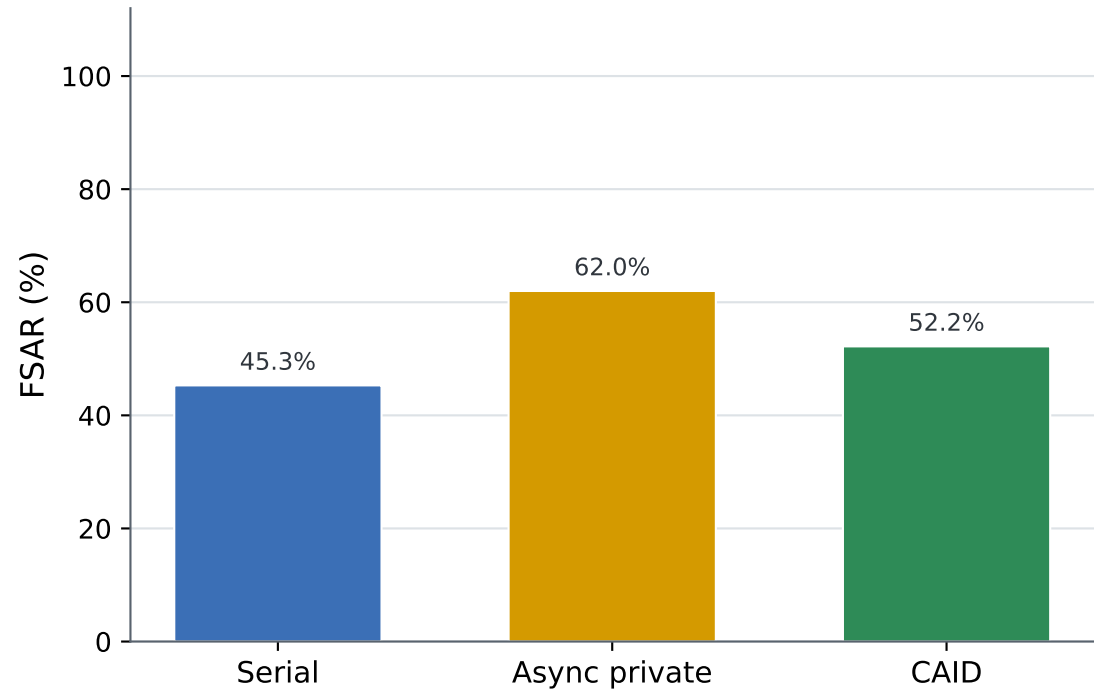
Failed subagent attempts (lower is better)
