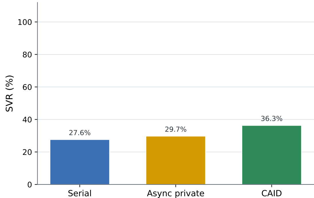
Writable-scope violations (lower is better)
