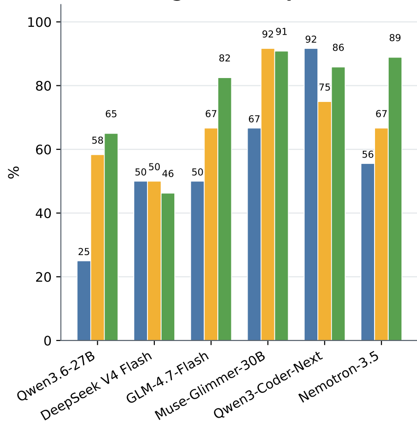
Failed subagent attempts — FSAR ↓
