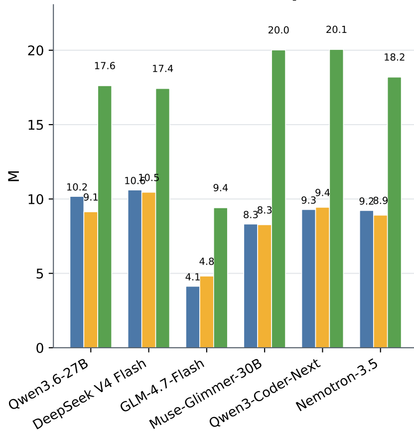
Mean model tokens per cell ↓
