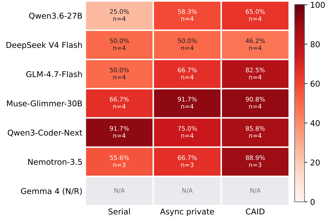
Failed attempts — FSAR ↓
