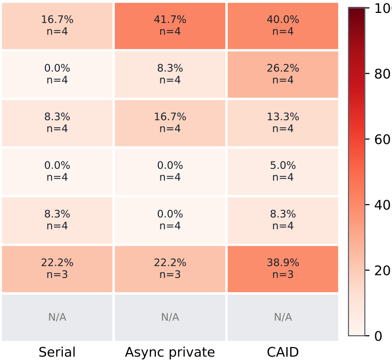
Scope violations — SVR ↓
