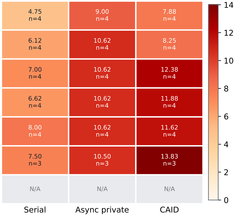
Integration lag — CAIL-P ↓
