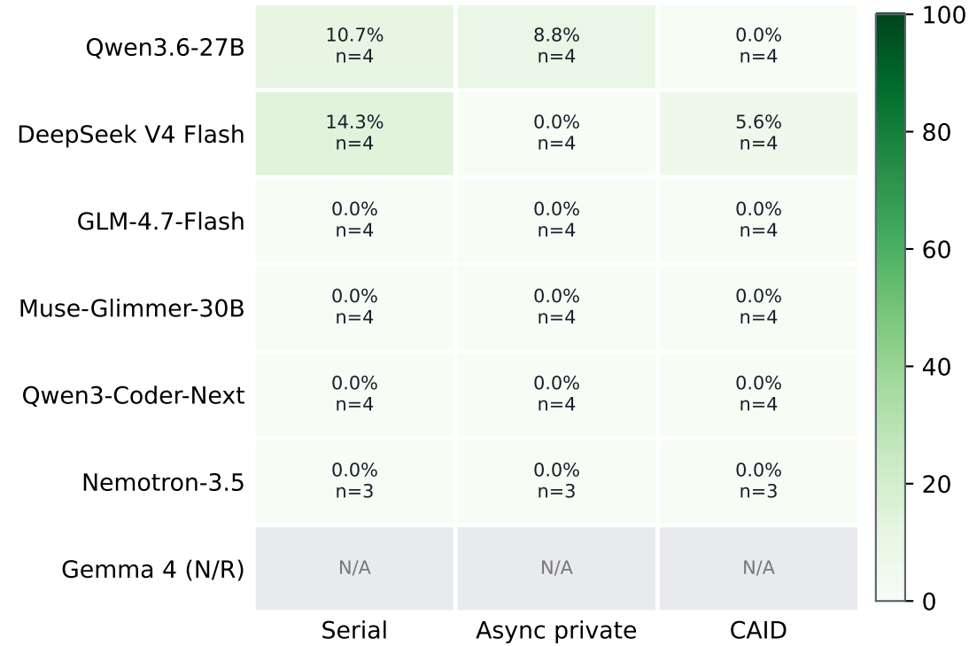
Resolution efficiency — DRE ↑
