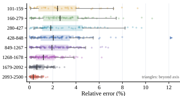
(f) Peak-response relative error
