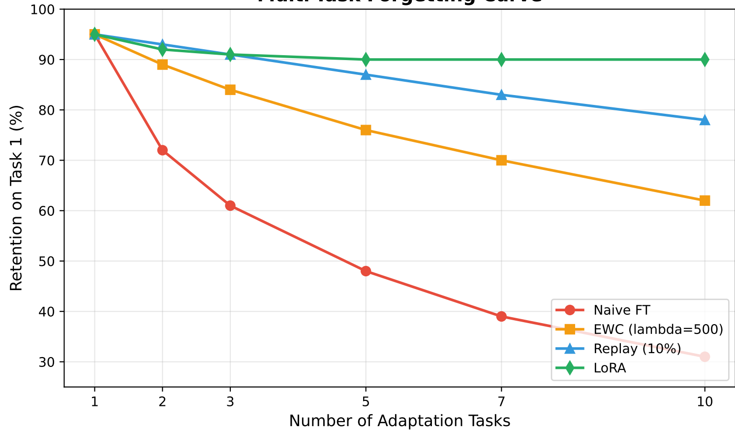
Multi-Task Forgetting Curve
