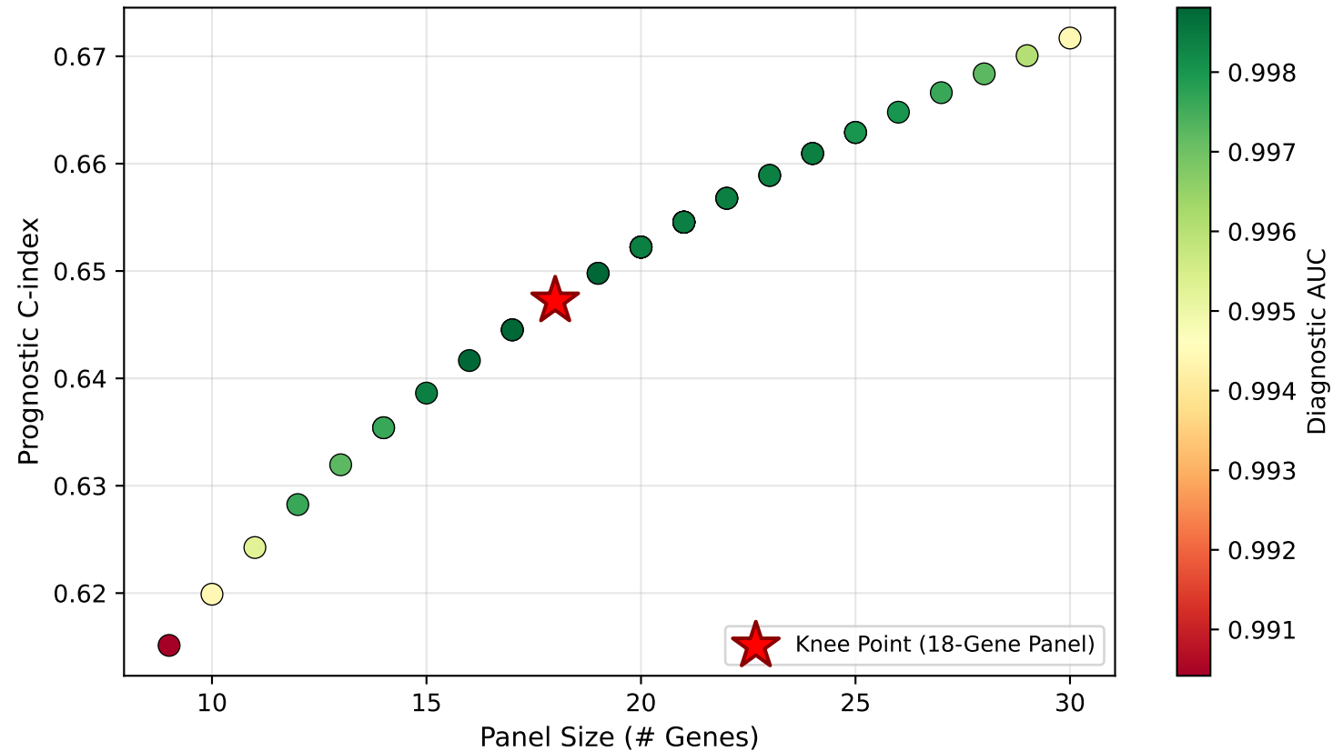
NSGA-II Pareto Frontier (Diagnostic AUC × Prognostic C-index × Panel Size)
