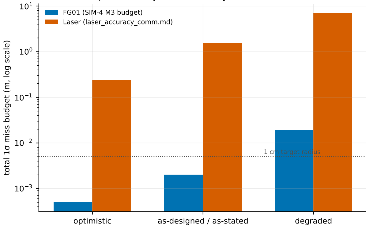
SIM-14: terminal miss budget, three scenarios each (scope: accuracy tolerance only -- see SIM-9 for cost)
