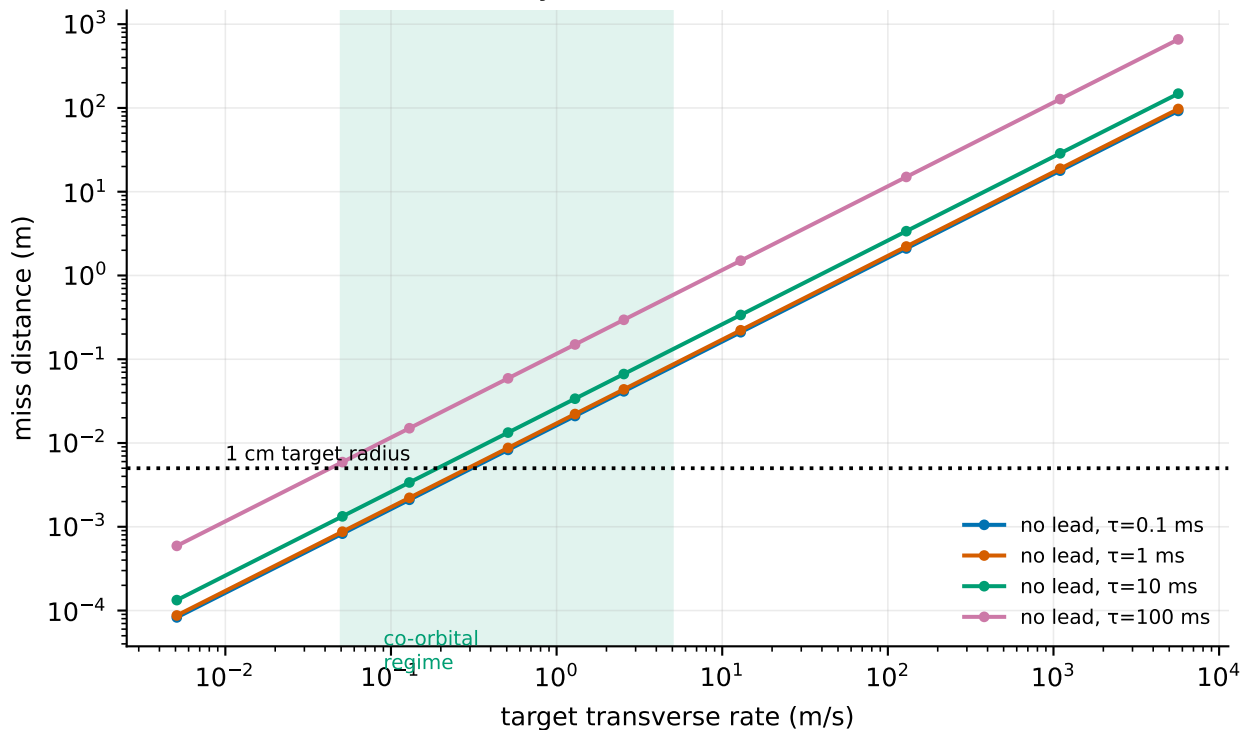
INT-0: where the latency term does and does not bite ( R = 10 m)
